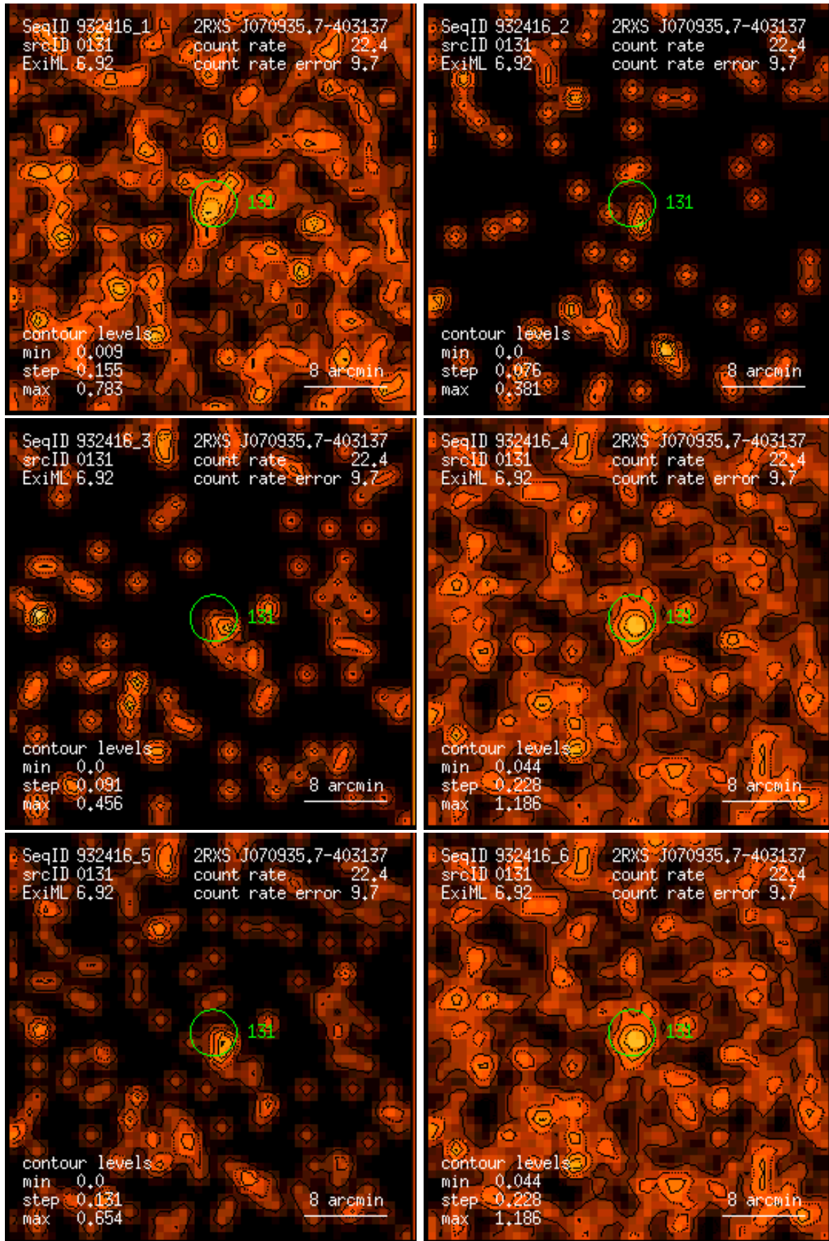
Figure 131: RASS 932416: detection 0131: band rate images, Gaussian filter: (1) PSPC channels 11 – 41, (2) 52 – 90, (3) 91 – 201, (4) 11 – 235, (5) 52 – 201, (6) 11 – 201. Broad band rates in counts/ks. Band rate contour levels in counts/ks/arcmin 2 .
