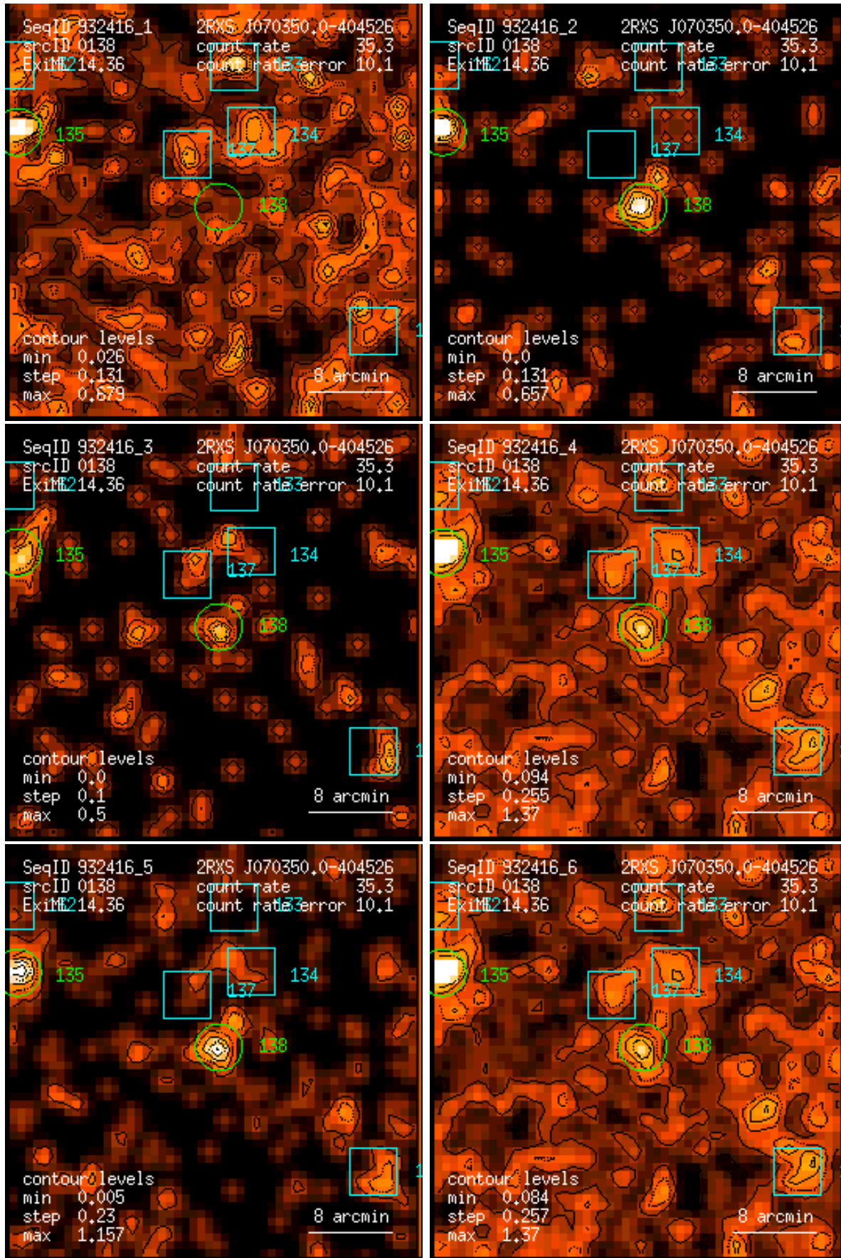
Figure 138: RASS 932416: detection 0138: band rate images, Gaussian filter: (1) PSPC channels 11 – 41, (2) 52 – 90, (3) 91 – 201, (4) 11 – 235, (5) 52 – 201, (6) 11 – 201. Broad band rates in counts/ks. Band rate contour levels in counts/ks/arcmin 2 .
