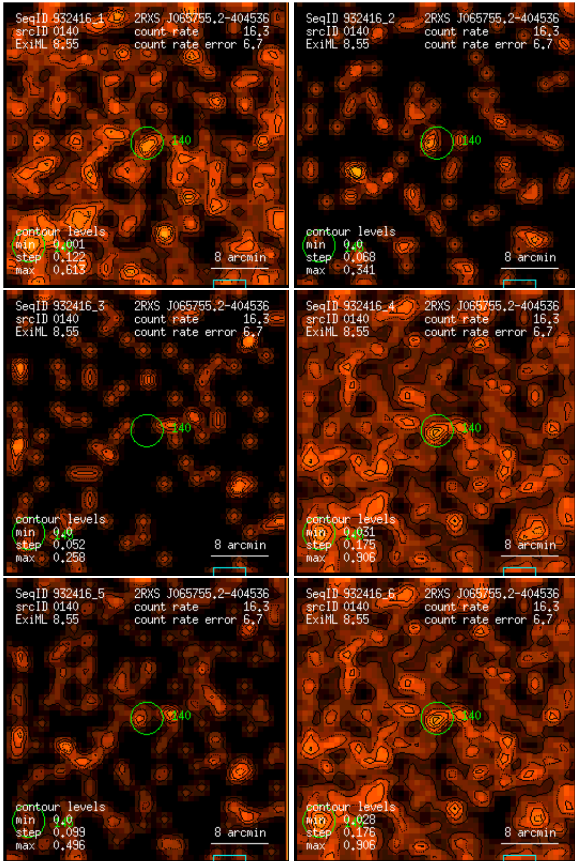
Figure 140: RASS 932416: detection 0140: band rate images, Gaussian filter: (1) PSPC channels 11 – 41, (2) 52 – 90, (3) 91 – 201, (4) 11 – 235, (5) 52 – 201, (6) 11 – 201. Broad band rates in counts/ks. Band rate contour levels in counts/ks/arcmin 2 .
