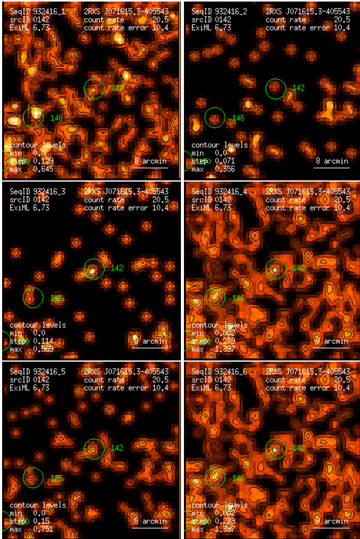
Figure 142: RASS 932416: detection 0142: band rate images, Gaussian filter: (1) PSPC channels 11 – 41, (2) 52 – 90, (3) 91 – 201, (4) 11 – 235, (5) 52 – 201, (6) 11 – 201. Broad band rates in counts/ks. Band rate contour levels in counts/ks/arcmin 2 .
