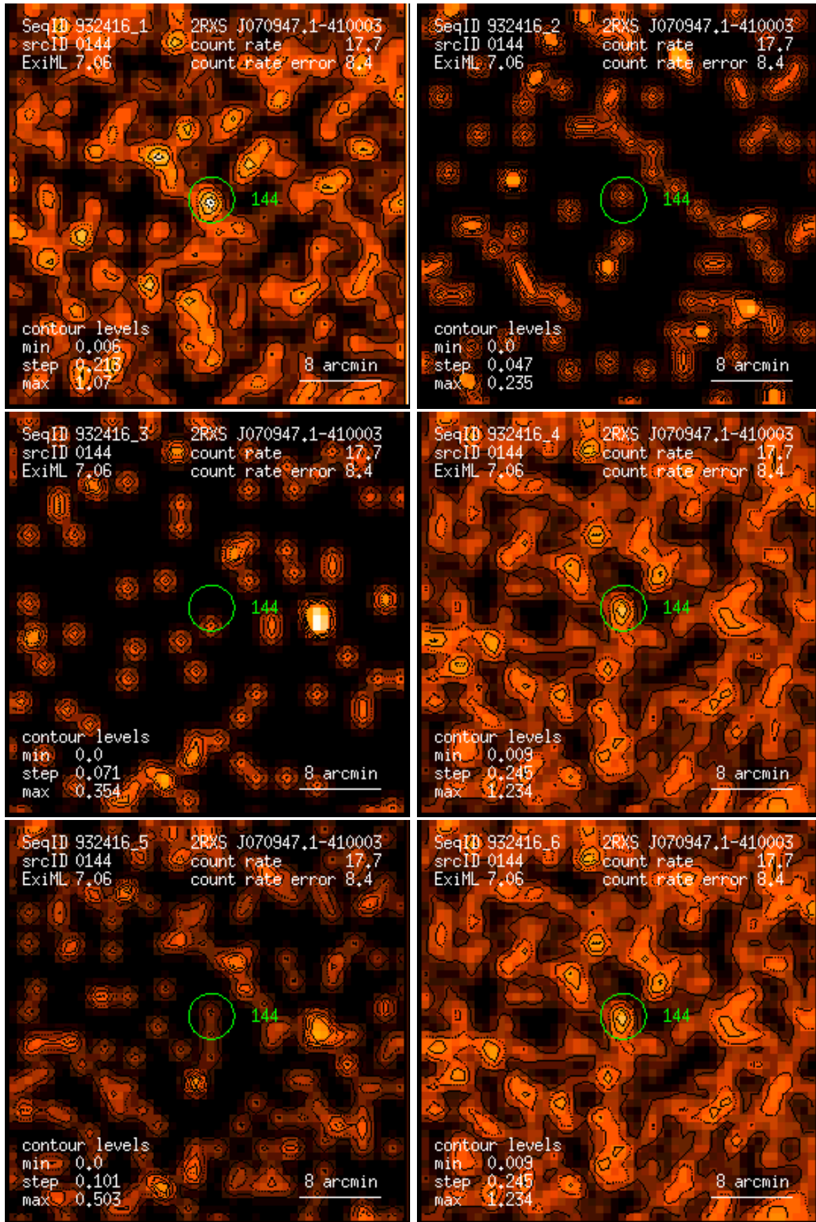
Figure 144: RASS 932416: detection 0144: band rate images, Gaussian filter: (1) PSPC channels 11 – 41, (2) 52 – 90, (3) 91 – 201, (4) 11 – 235, (5) 52 – 201, (6) 11 – 201. Broad band rates in counts/ks. Band rate contour levels in counts/ks/arcmin 2 .
