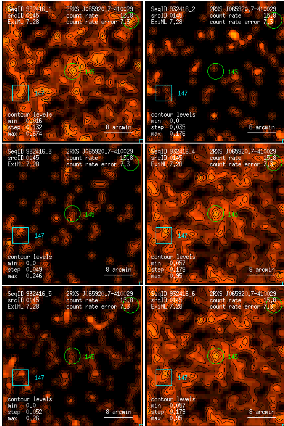
Figure 145: RASS 932416: detection 0145: band rate images, Gaussian filter: (1) PSPC channels 11 – 41, (2) 52 – 90, (3) 91 – 201, (4) 11 – 235, (5) 52 – 201, (6) 11 – 201. Broad band rates in counts/ks. Band rate contour levels in counts/ks/arcmin 2 .
