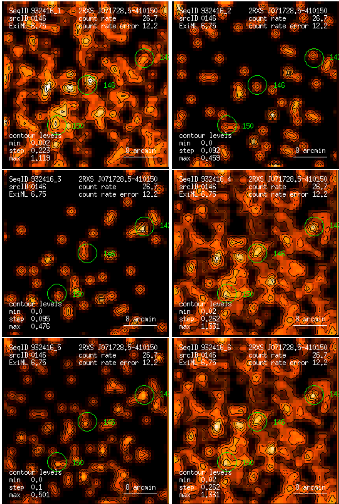
Figure 146: RASS 932416: detection 0146: band rate images, Gaussian filter: (1) PSPC channels 11 – 41, (2) 52 – 90, (3) 91 – 201, (4) 11 – 235, (5) 52 – 201, (6) 11 – 201. Broad band rates in counts/ks. Band rate contour levels in counts/ks/arcmin 2 .
