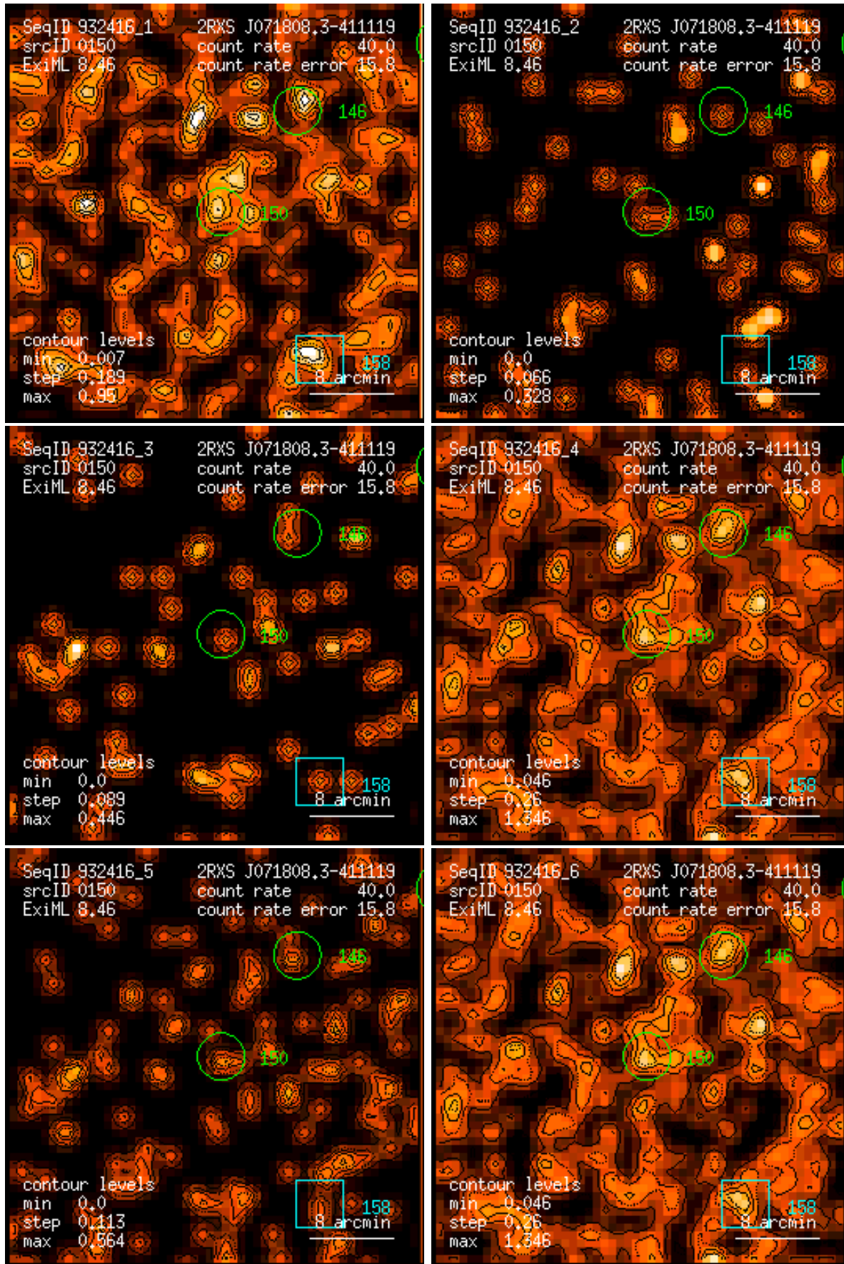
Figure 150: RASS 932416: detection 0150: band rate images, Gaussian filter: (1) PSPC channels 11 – 41, (2) 52 – 90, (3) 91 – 201, (4) 11 – 235, (5) 52 – 201, (6) 11 – 201. Broad band rates in counts/ks. Band rate contour levels in counts/ks/arcmin 2 .
