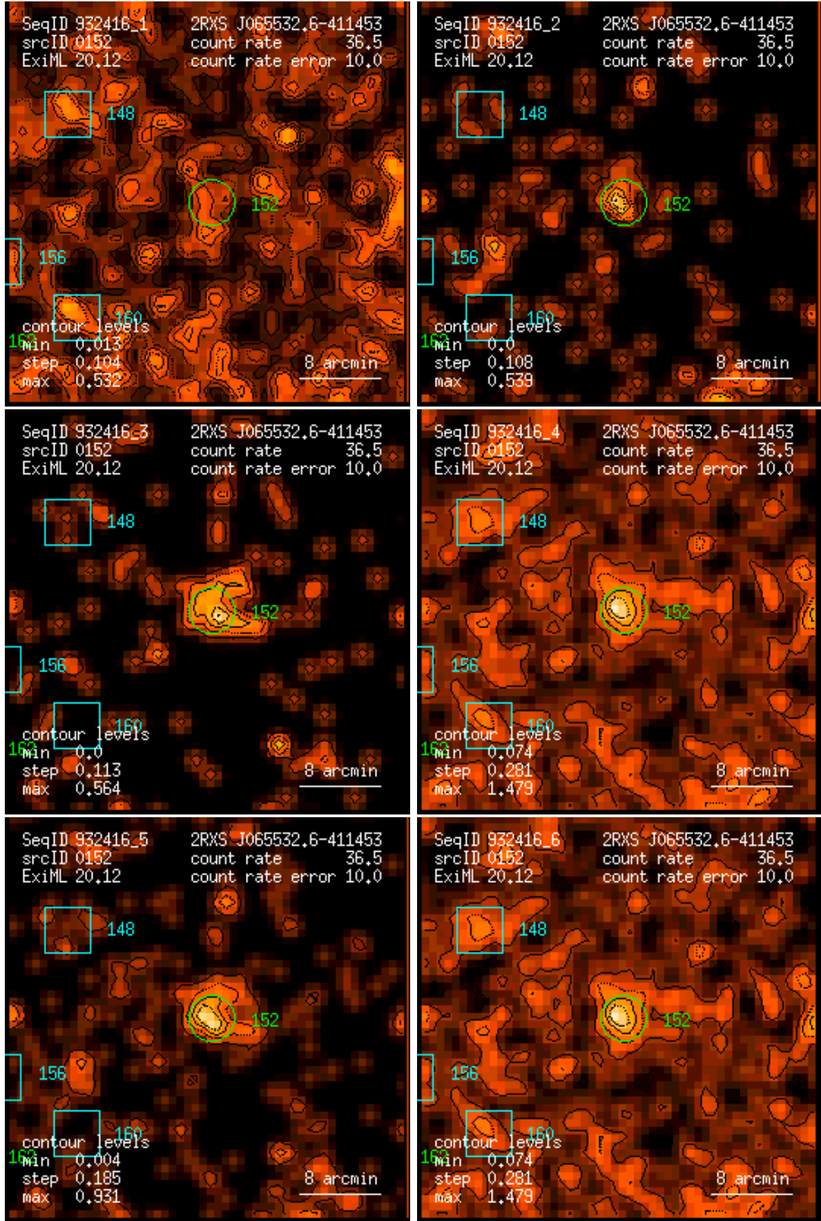
Figure 152: RASS 932416: detection 0152: band rate images, Gaussian filter: (1) PSPC channels 11 – 41, (2) 52 – 90, (3) 91 – 201, (4) 11 – 235, (5) 52 – 201, (6) 11 – 201. Broad band rates in counts/ks. Band rate contour levels in counts/ks/arcmin 2 .
