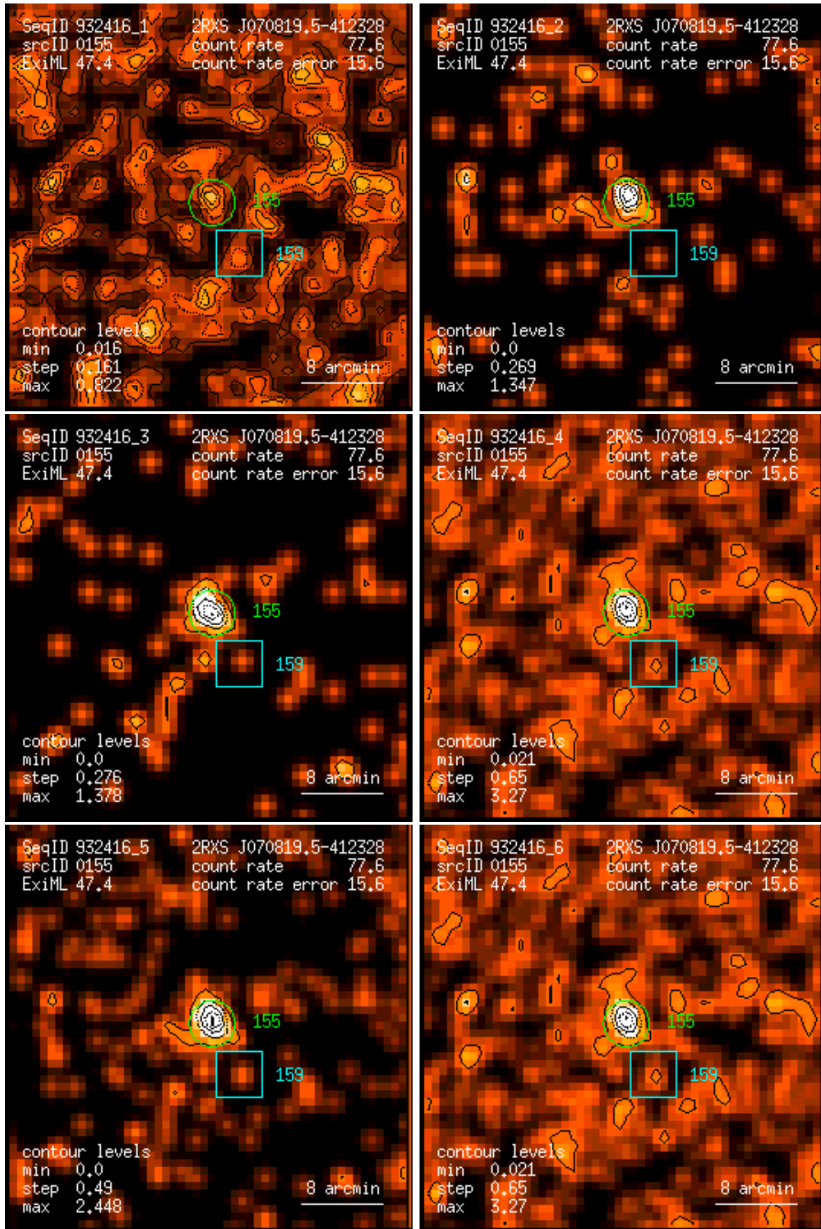
Figure 155: RASS 932416: detection 0155: band rate images, Gaussian filter: (1) PSPC channels 11 – 41, (2) 52 – 90, (3) 91 – 201, (4) 11 – 235, (5) 52 – 201, (6) 11 – 201. Broad band rates in counts/ks. Band rate contour levels in counts/ks/arcmin 2 .
