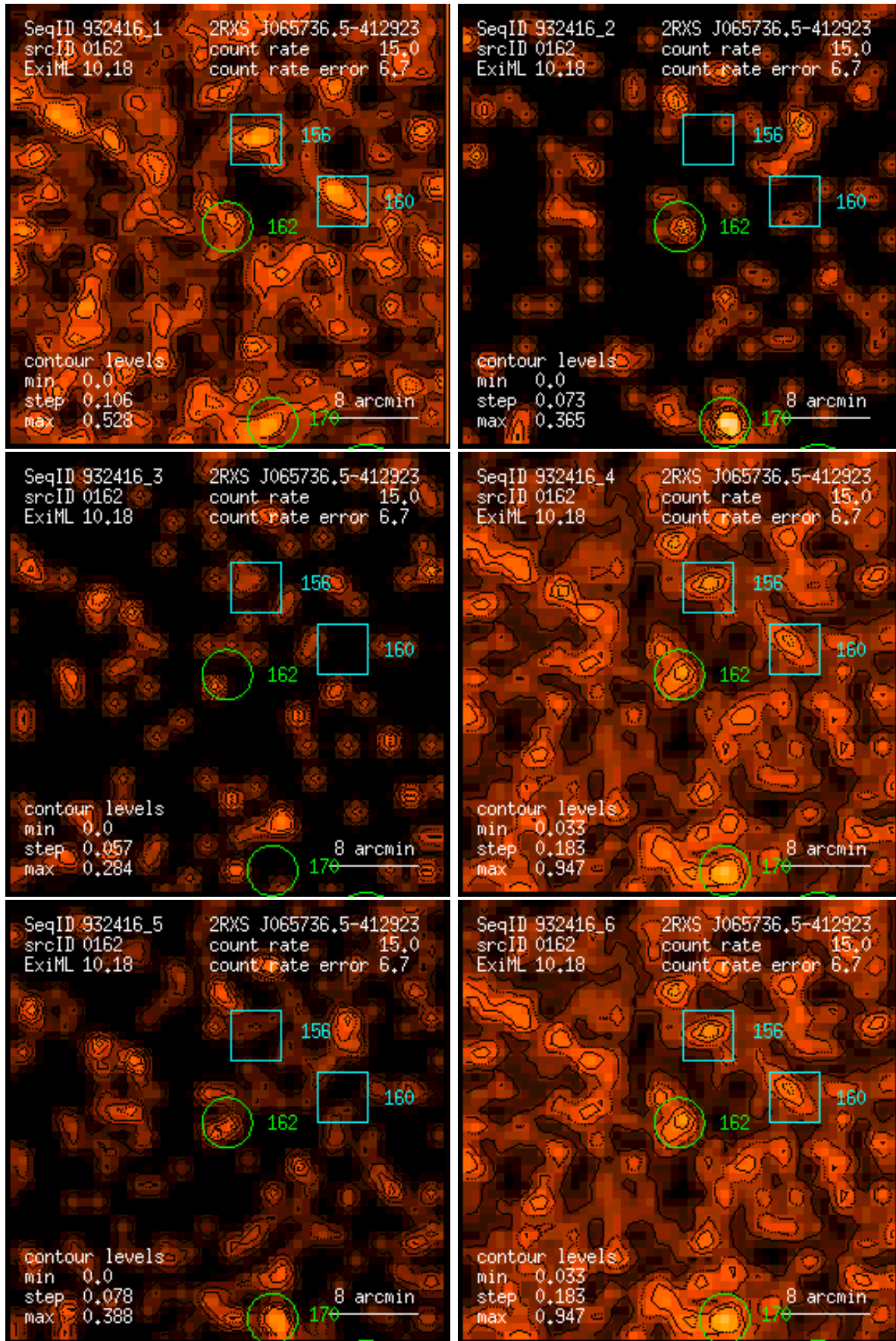
Figure 162: RASS 932416: detection 0162: band rate images, Gaussian filter: (1) PSPC channels 11 – 41, (2) 52 – 90, (3) 91 – 201, (4) 11 – 235, (5) 52 – 201, (6) 11 – 201. Broad band rates in counts/ks. Band rate contour levels in counts/ks/arcmin 2 .
