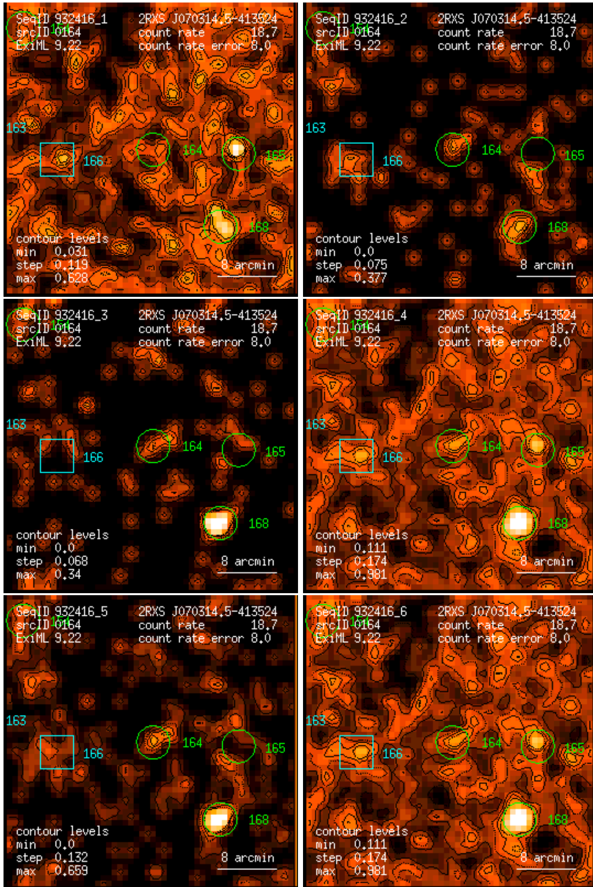
Figure 164: RASS 932416: detection 0164: band rate images, Gaussian filter: (1) PSPC channels 11 – 41, (2) 52 – 90, (3) 91 – 201, (4) 11 – 235, (5) 52 – 201, (6) 11 – 201. Broad band rates in counts/ks. Band rate contour levels in counts/ks/arcmin 2 .
