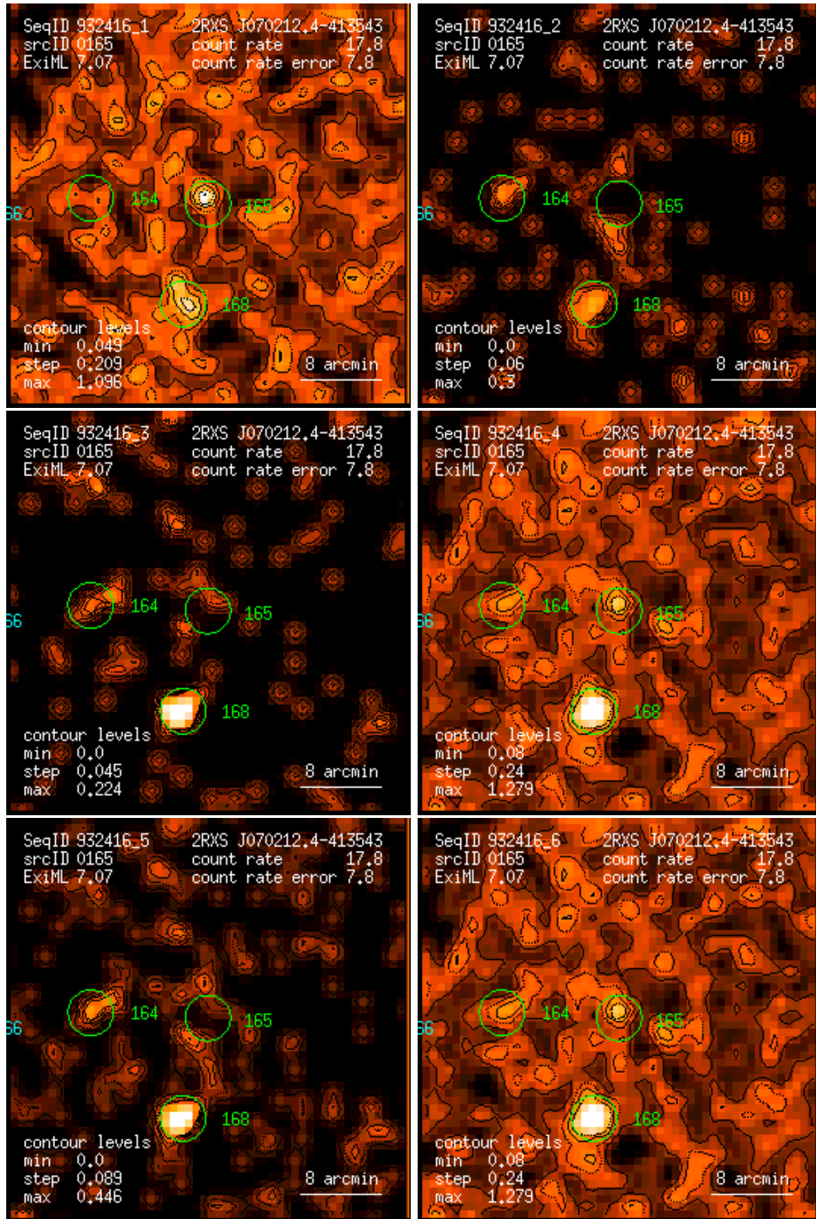
Figure 165: RASS 932416: detection 0165: band rate images, Gaussian filter: (1) PSPC channels 11 – 41, (2) 52 – 90, (3) 91 – 201, (4) 11 – 235, (5) 52 – 201, (6) 11 – 201. Broad band rates in counts/ks. Band rate contour levels in counts/ks/arcmin 2 .
