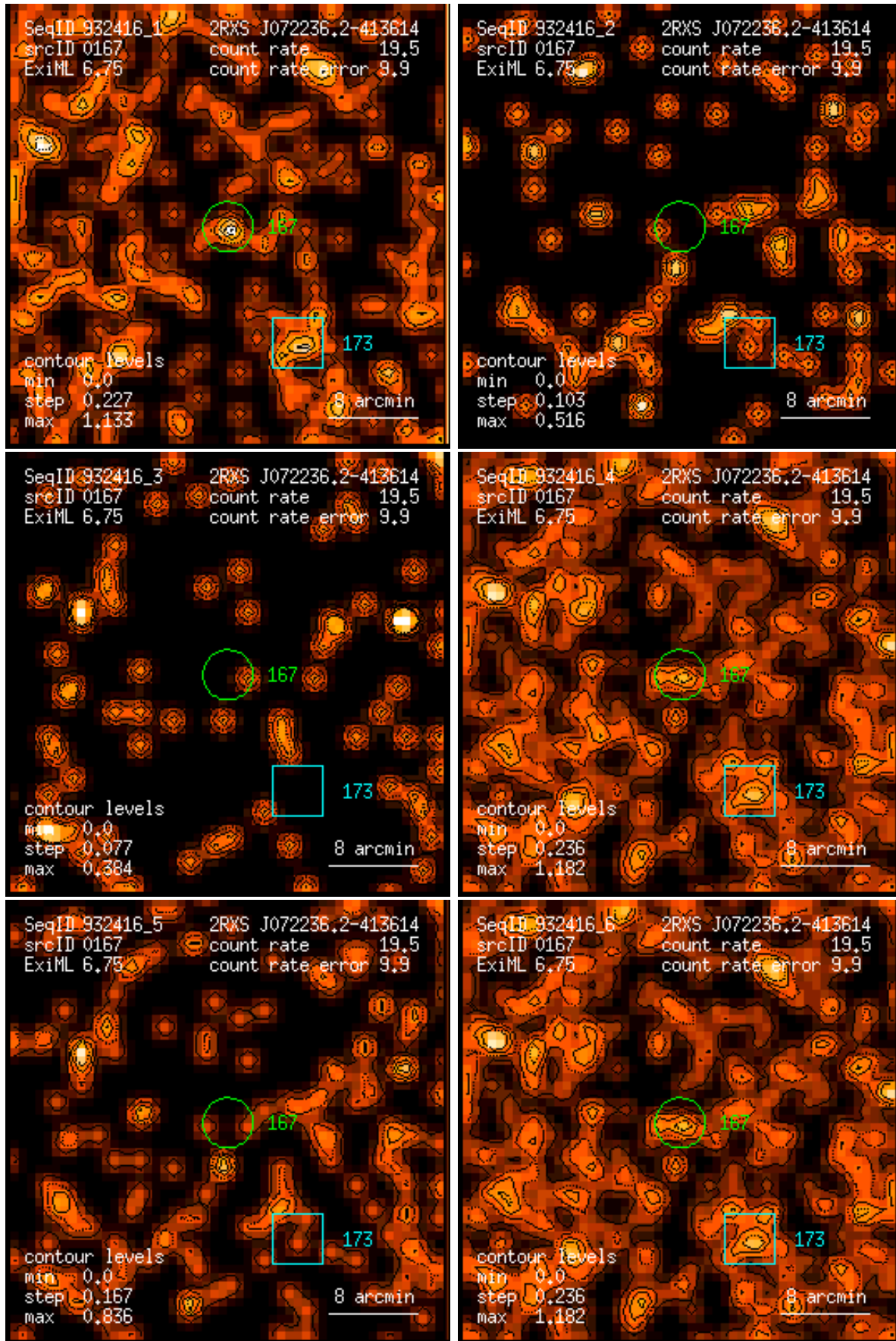
Figure 167: RASS 932416: detection 0167: band rate images, Gaussian filter: (1) PSPC channels 11 – 41, (2) 52 – 90, (3) 91 – 201, (4) 11 – 235, (5) 52 – 201, (6) 11 – 201. Broad band rates in counts/ks. Band rate contour levels in counts/ks/arcmin 2 .
