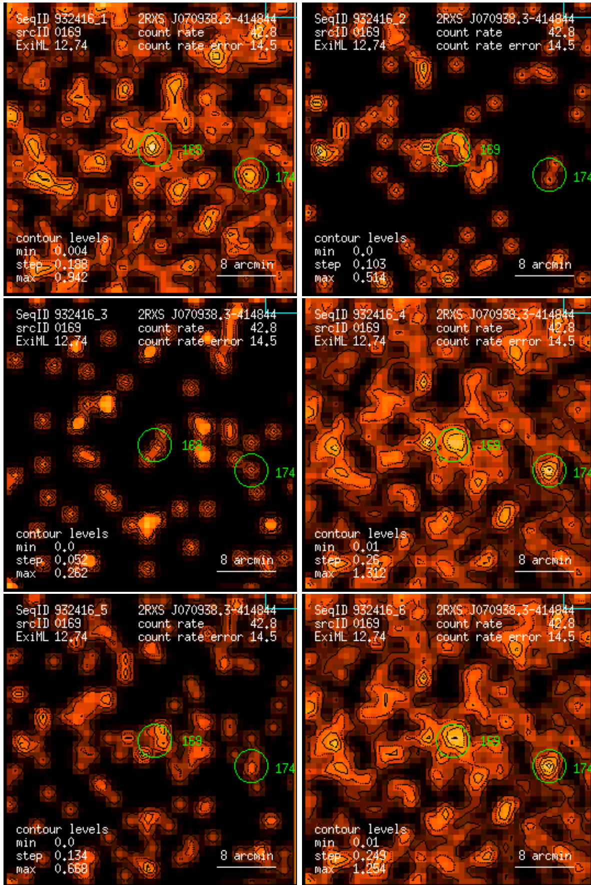
Figure 169: RASS 932416: detection 0169: band rate images, Gaussian filter: (1) PSPC channels 11 – 41, (2) 52 – 90, (3) 91 – 201, (4) 11 – 235, (5) 52 – 201, (6) 11 – 201. Broad band rates in counts/ks. Band rate contour levels in counts/ks/arcmin 2 .
