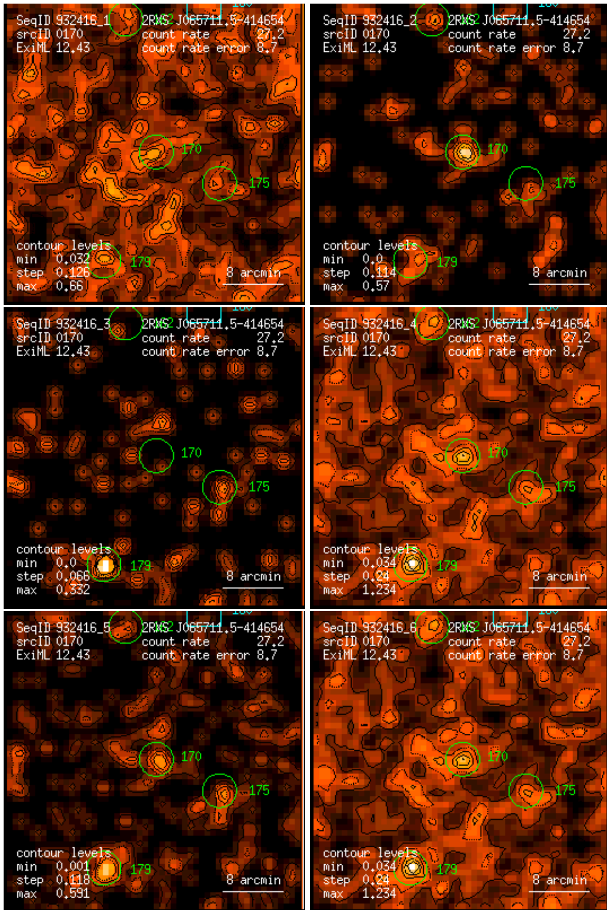
Figure 170: RASS 932416: detection 0170: band rate images, Gaussian filter: (1) PSPC channels 11 – 41, (2) 52 – 90, (3) 91 – 201, (4) 11 – 235, (5) 52 – 201, (6) 11 – 201. Broad band rates in counts/ks. Band rate contour levels in counts/ks/arcmin 2 .
