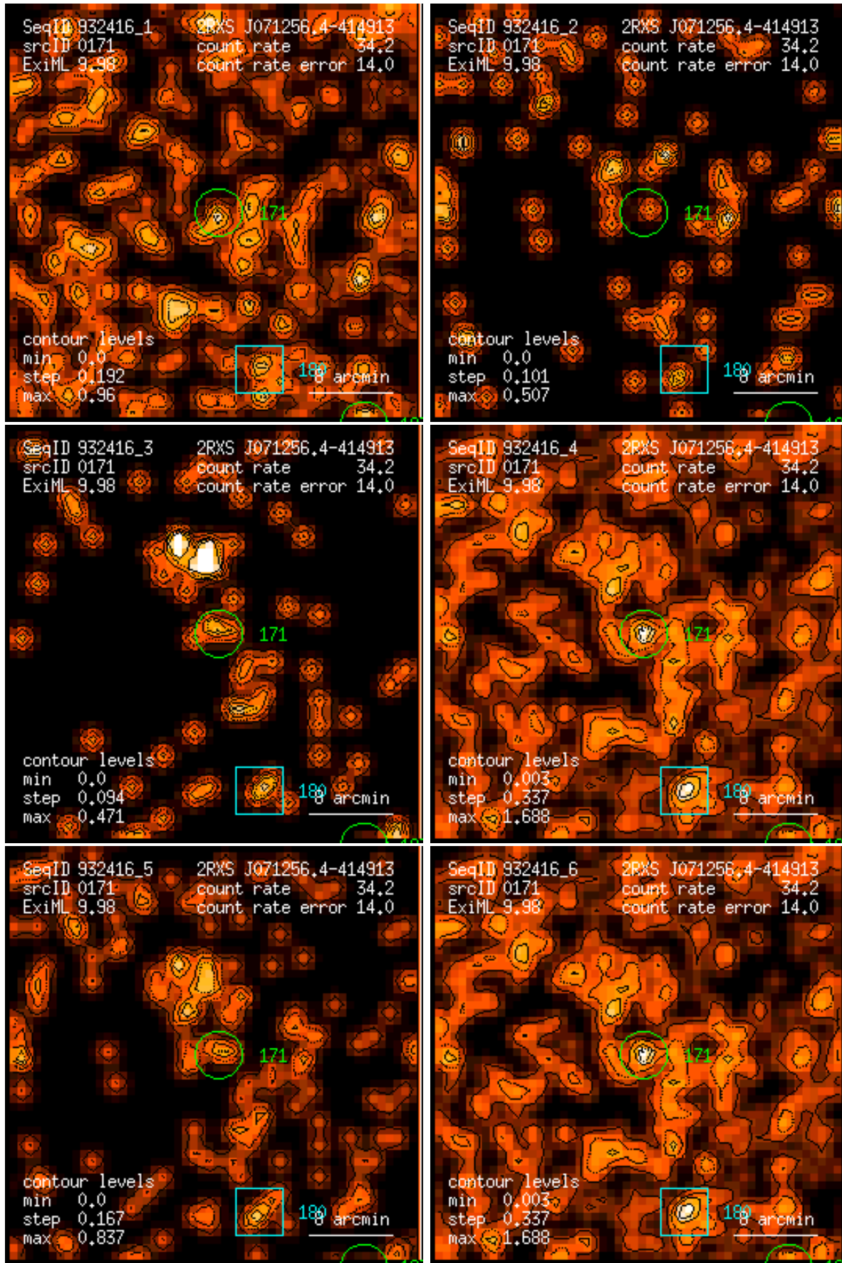
Figure 171: RASS 932416: detection 0171: band rate images, Gaussian filter: (1) PSPC channels 11 – 41, (2) 52 – 90, (3) 91 – 201, (4) 11 – 235, (5) 52 – 201, (6) 11 – 201. Broad band rates in counts/ks. Band rate contour levels in counts/ks/arcmin 2 .
