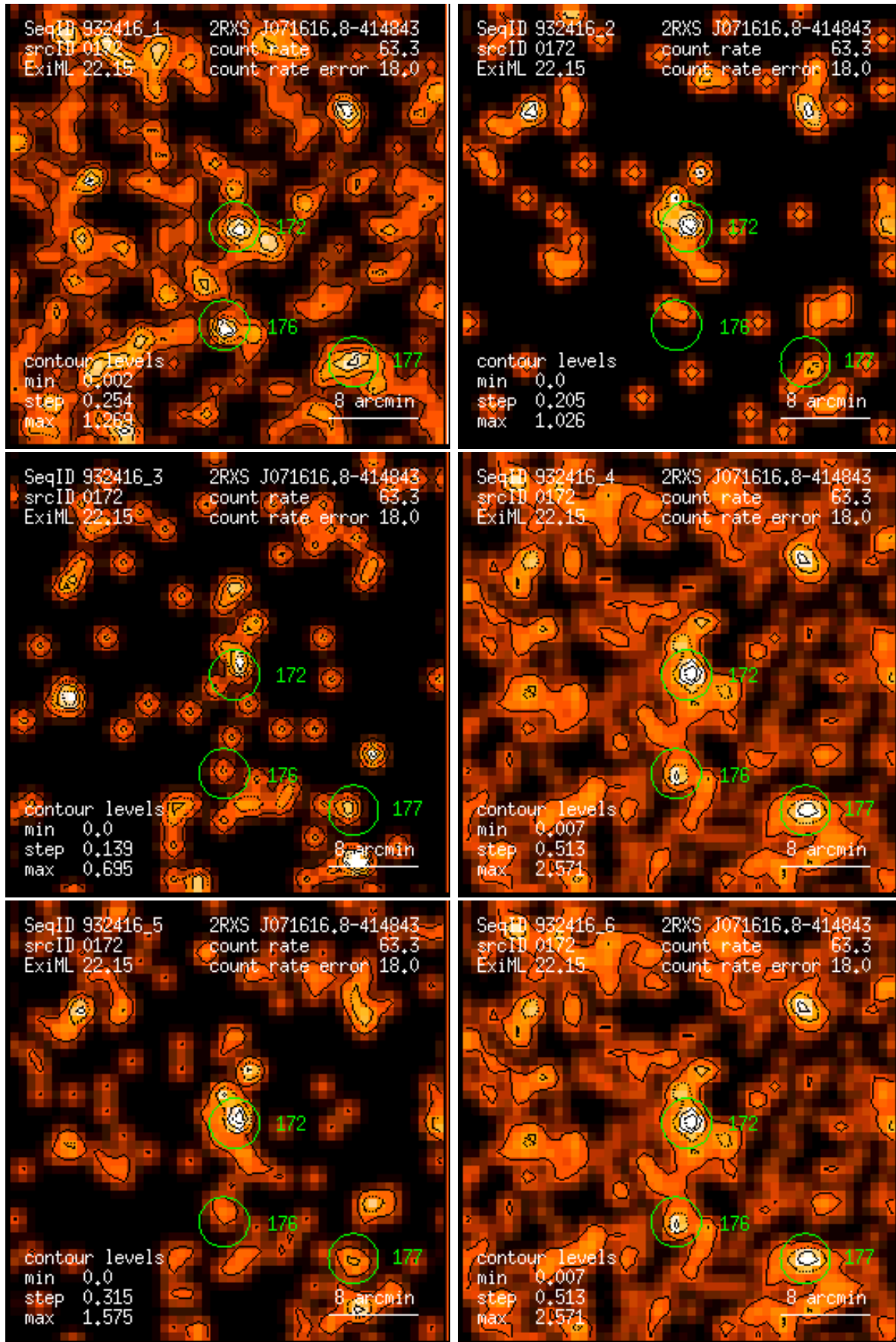
Figure 172: RASS 932416: detection 0172: band rate images, Gaussian filter: (1) PSPC channels 11 – 41, (2) 52 – 90, (3) 91 – 201, (4) 11 – 235, (5) 52 – 201, (6) 11 – 201. Broad band rates in counts/ks. Band rate contour levels in counts/ks/arcmin 2 .
