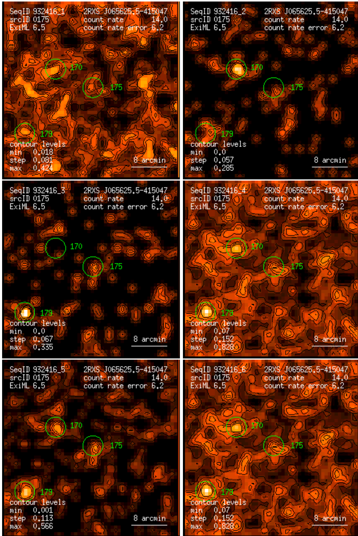
Figure 175: RASS 932416: detection 0175: band rate images, Gaussian filter: (1) PSPC channels 11 – 41, (2) 52 – 90, (3) 91 – 201, (4) 11 – 235, (5) 52 – 201, (6) 11 – 201. Broad band rates in counts/ks. Band rate contour levels in counts/ks/arcmin 2 .
