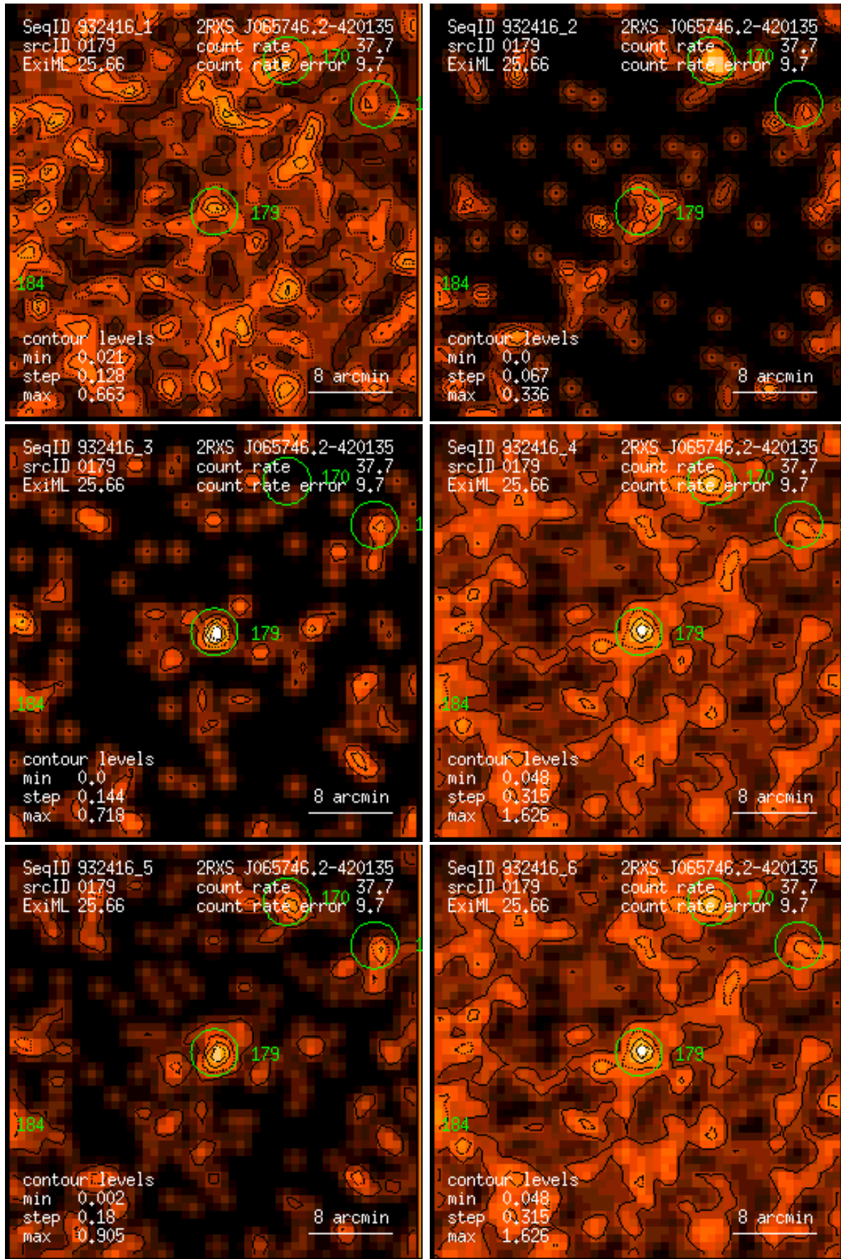
Figure 179: RASS 932416: detection 0179: band rate images, Gaussian filter: (1) PSPC channels 11 – 41, (2) 52 – 90, (3) 91 – 201, (4) 11 – 235, (5) 52 – 201, (6) 11 – 201. Broad band rates in counts/ks. Band rate contour levels in counts/ks/arcmin 2 .
