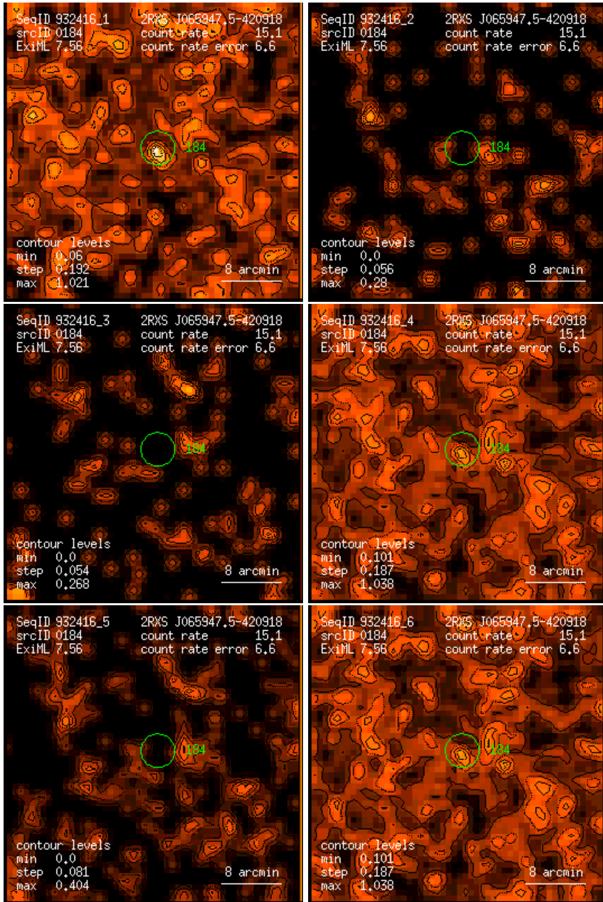
Figure 184: RASS 932416: detection 0184: band rate images, Gaussian filter: (1) PSPC channels 11 – 41, (2) 52 – 90, (3) 91 – 201, (4) 11 – 235, (5) 52 – 201, (6) 11 – 201. Broad band rates in counts/ks. Band rate contour levels in counts/ks/arcmin 2 .
