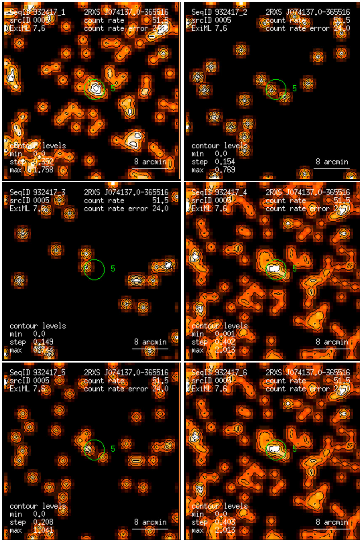
Figure 5: RASS 932417: detection 0005: band rate images, Gaussian filter: (1) PSPC channels 11 – 41, (2) 52 – 90, (3) 91 – 201, (4) 11 – 235, (5) 52 – 201, (6) 11 – 201. Broad band rates in counts/ks. Band rate contour levels in counts/ks/arcmin 2 .
