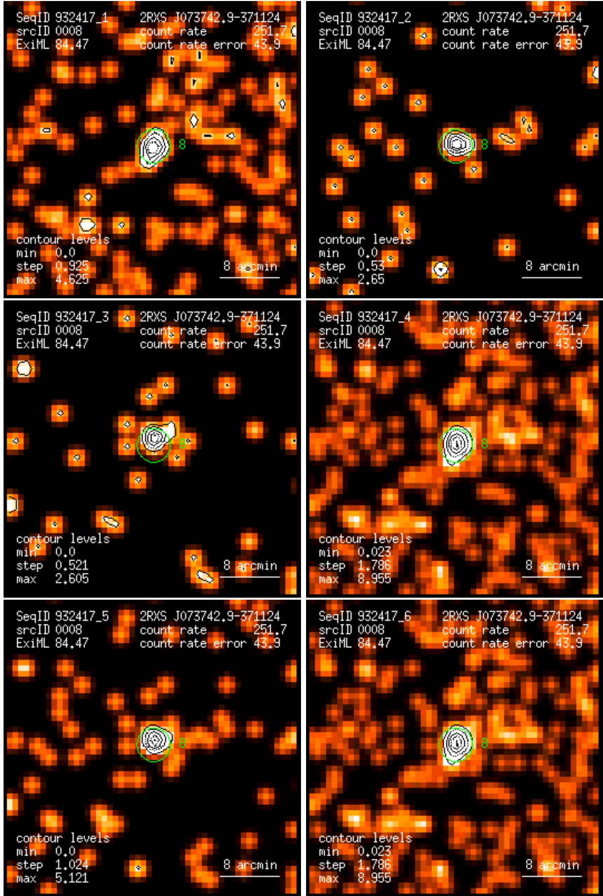
Figure 8: RASS 932417: detection 0008: band rate images, Gaussian filter: (1) PSPC channels 11 – 41, (2) 52 – 90, (3) 91 – 201, (4) 11 – 235, (5) 52 – 201, (6) 11 – 201. Broad band rates in counts/ks. Band rate contour levels in counts/ks/arcmin 2 .
