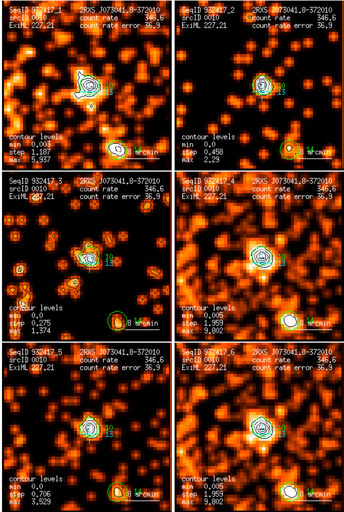
Figure 10: RASS 932417: detection 0010: band rate images, Gaussian filter: (1) PSPC channels 11 – 41, (2) 52 – 90, (3) 91 – 201, (4) 11 – 235, (5) 52 – 201, (6) 11 – 201. Broad band rates in counts/ks. Band rate contour levels in counts/ks/arcmin 2 .
