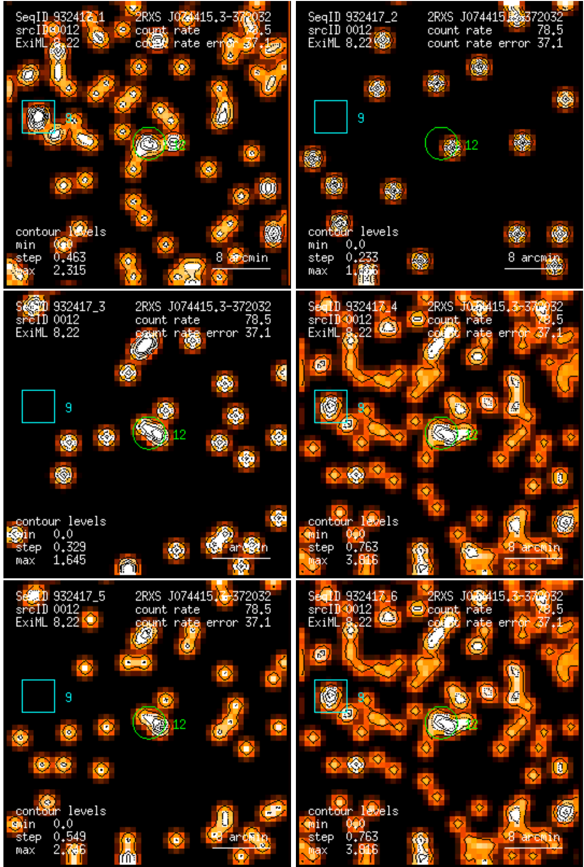
Figure 12: RASS 932417: detection 0012: band rate images, Gaussian filter: (1) PSPC channels 11 – 41, (2) 52 – 90, (3) 91 – 201, (4) 11 – 235, (5) 52 – 201, (6) 11 – 201. Broad band rates in counts/ks. Band rate contour levels in counts/ks/arcmin 2 .
