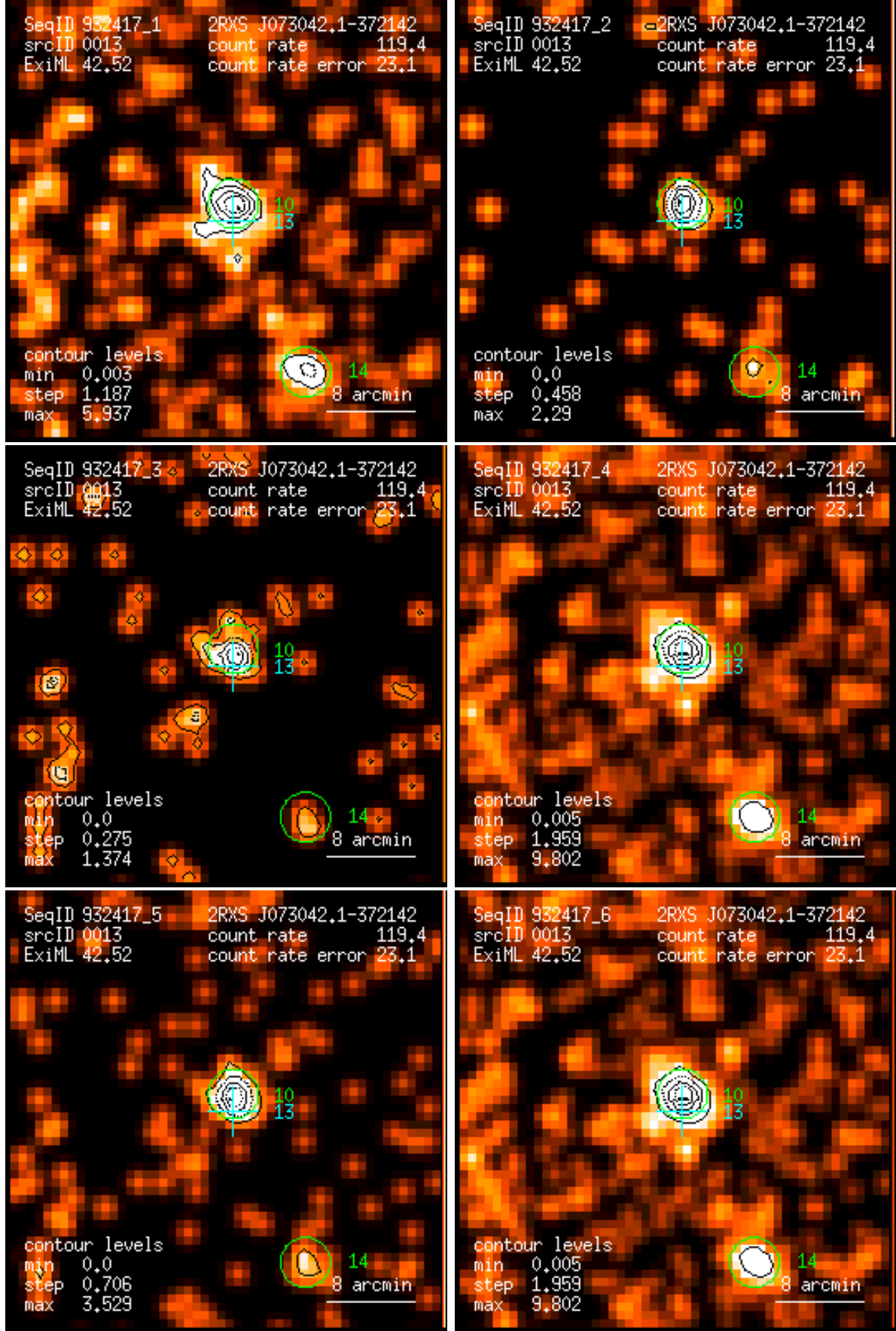
Figure 13: RASS 932417: detection 0013: band rate images, Gaussian filter: (1) PSPC channels 11 – 41, (2) 52 – 90, (3) 91 – 201, (4) 11 – 235, (5) 52 – 201, (6) 11 – 201. Broad band rates in counts/ks. Band rate contour levels in counts/ks/arcmin 2 .
