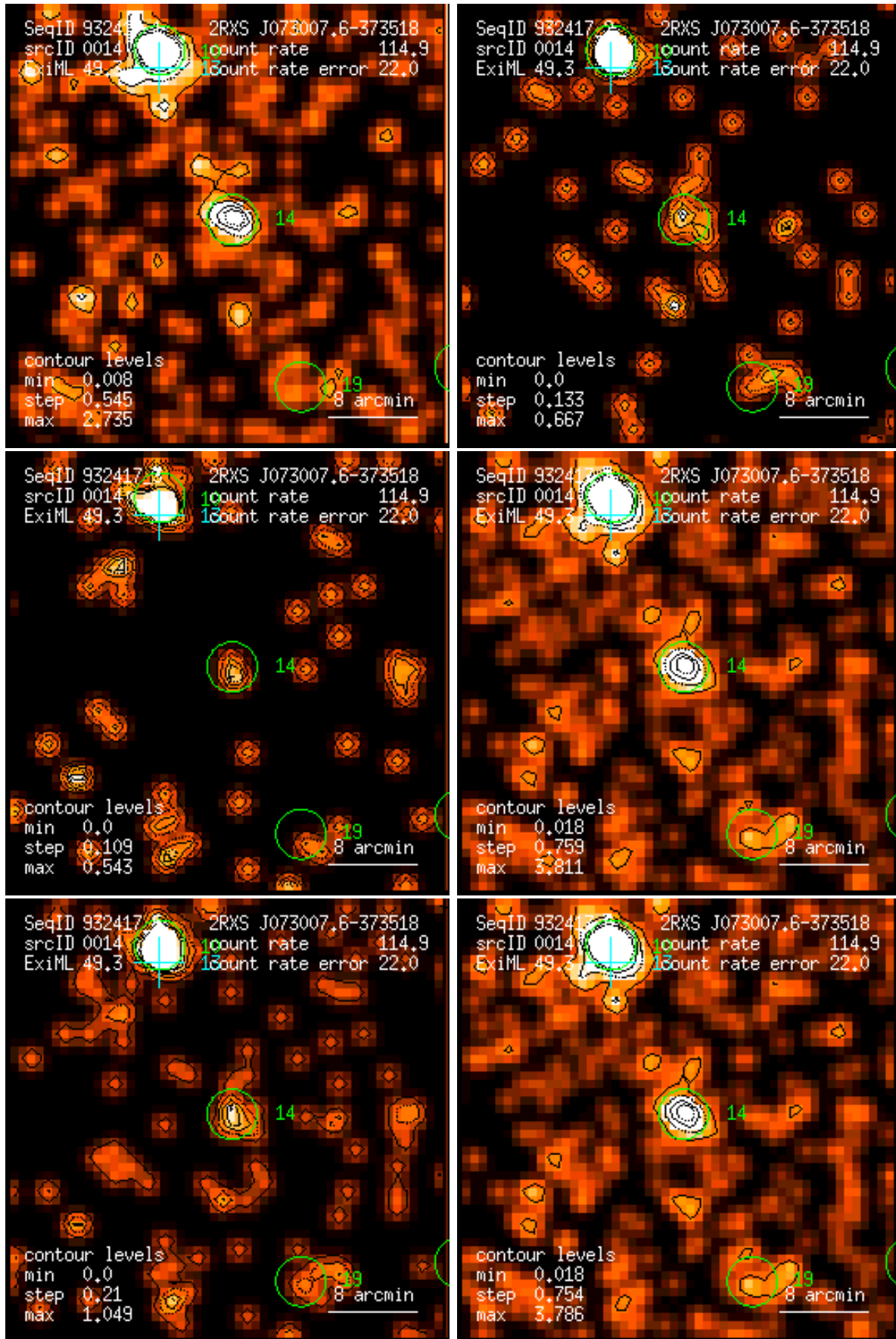
Figure 14: RASS 932417: detection 0014: band rate images, Gaussian filter: (1) PSPC channels 11 – 41, (2) 52 – 90, (3) 91 – 201, (4) 11 – 235, (5) 52 – 201, (6) 11 – 201. Broad band rates in counts/ks. Band rate contour levels in counts/ks/arcmin 2 .
