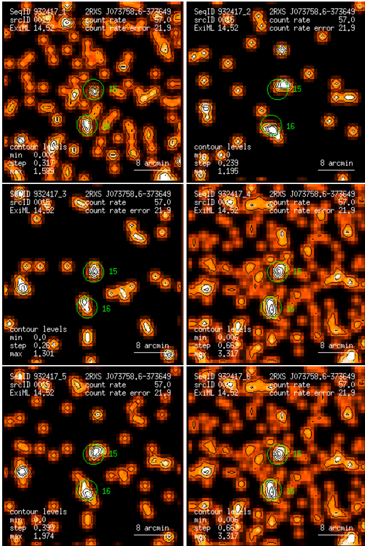
Figure 15: RASS 932417: detection 0015: band rate images, Gaussian filter: (1) PSPC channels 11 – 41, (2) 52 – 90, (3) 91 – 201, (4) 11 – 235, (5) 52 – 201, (6) 11 – 201. Broad band rates in counts/ks. Band rate contour levels in counts/ks/arcmin 2 .
