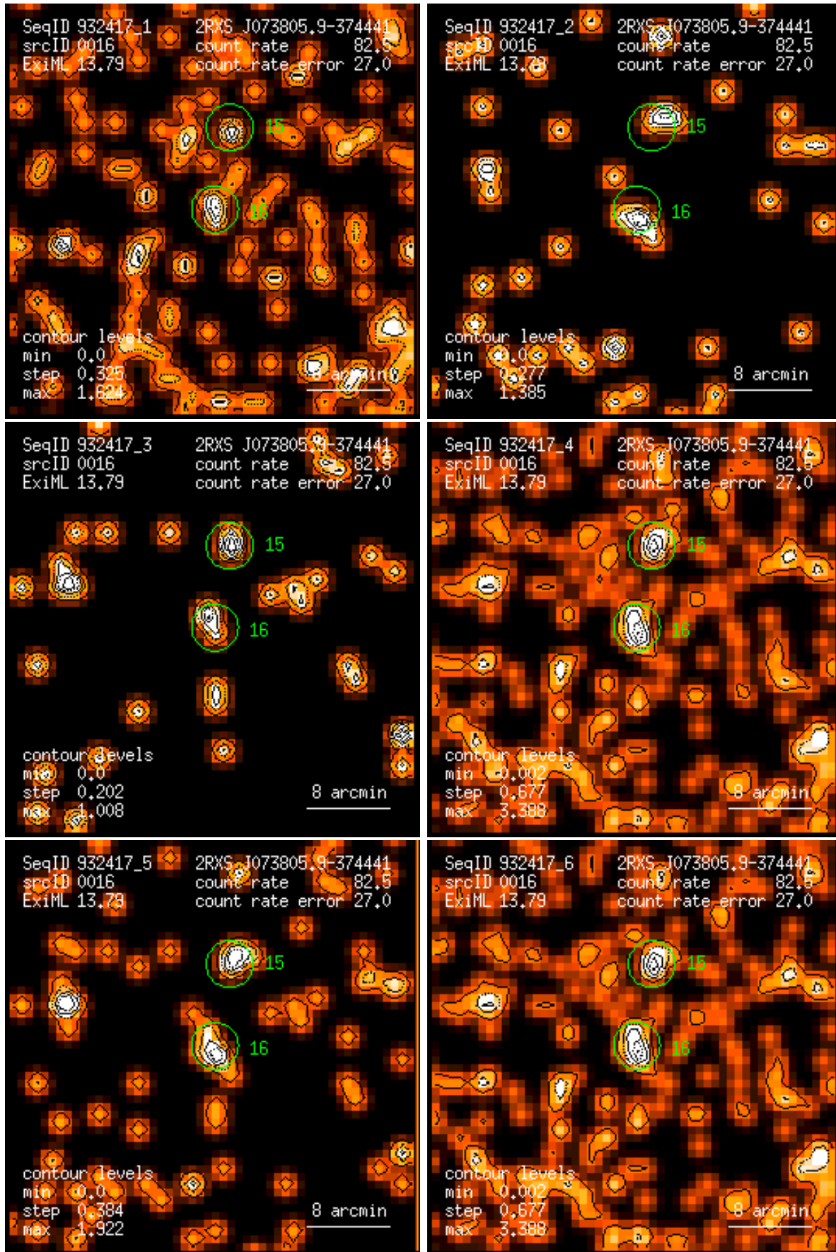
Figure 16: RASS 932417: detection 0016: band rate images, Gaussian filter: (1) PSPC channels 11 – 41, (2) 52 – 90, (3) 91 – 201, (4) 11 – 235, (5) 52 – 201, (6) 11 – 201. Broad band rates in counts/ks. Band rate contour levels in counts/ks/arcmin 2 .
