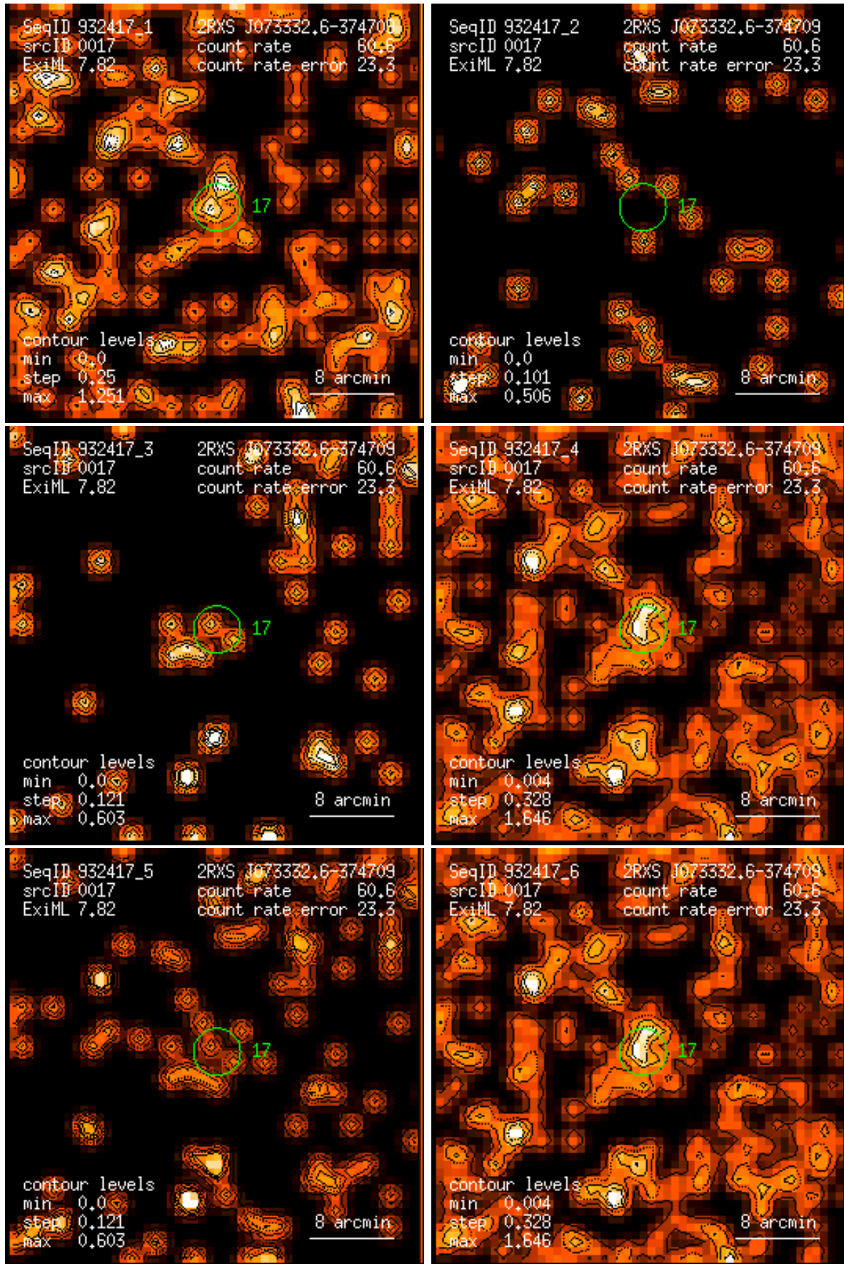
Figure 17: RASS 932417: detection 0017: band rate images, Gaussian filter: (1) PSPC channels 11 – 41, (2) 52 – 90, (3) 91 – 201, (4) 11 – 235, (5) 52 – 201, (6) 11 – 201. Broad band rates in counts/ks. Band rate contour levels in counts/ks/arcmin 2 .
