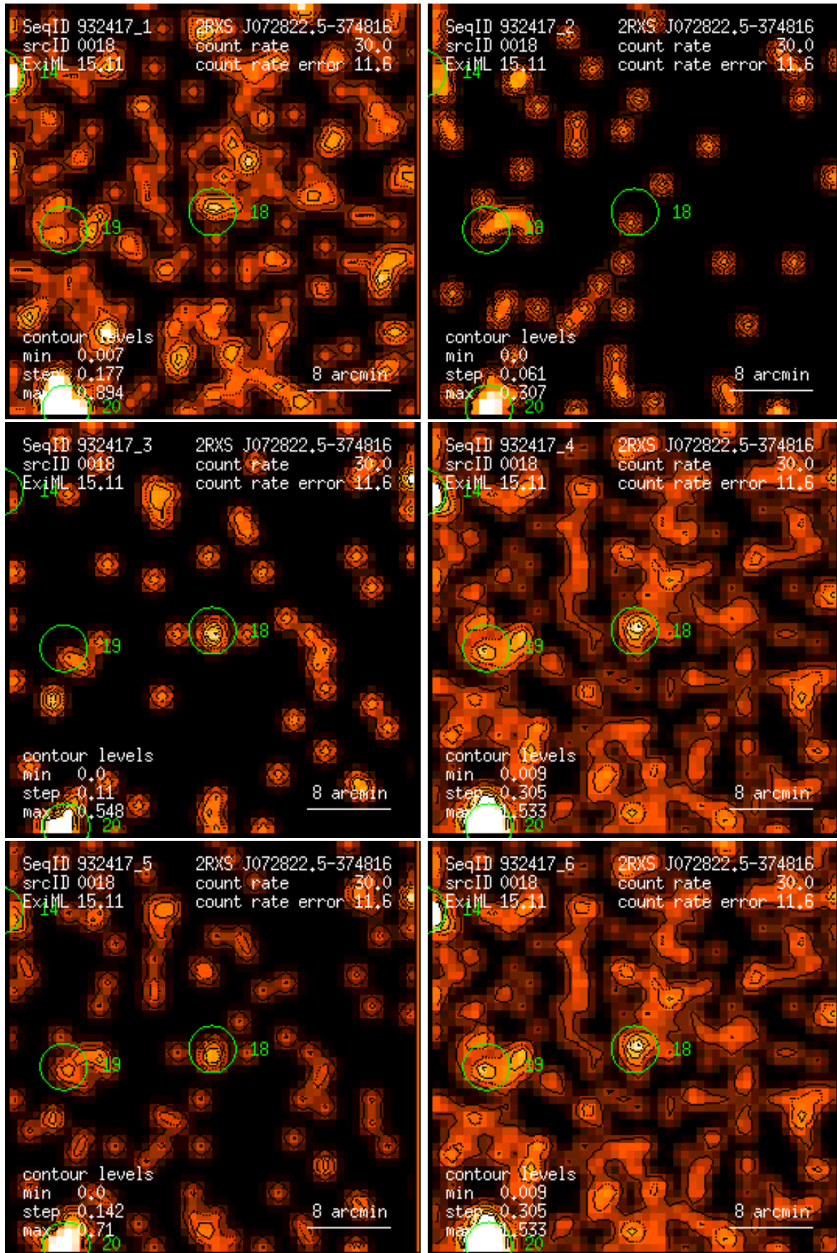
Figure 18: RASS 932417: detection 0018: band rate images, Gaussian filter: (1) PSPC channels 11 – 41, (2) 52 – 90, (3) 91 – 201, (4) 11 – 235, (5) 52 – 201, (6) 11 – 201. Broad band rates in counts/ks. Band rate contour levels in counts/ks/arcmin 2 .
