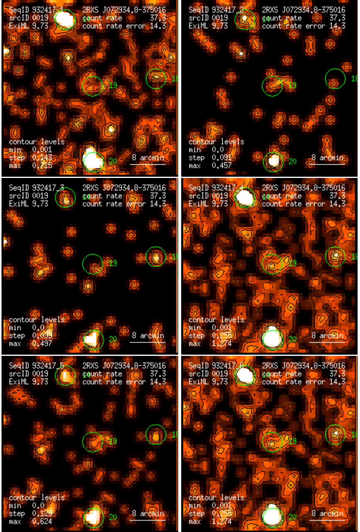
Figure 19: RASS 932417: detection 0019: band rate images, Gaussian filter: (1) PSPC channels 11 – 41, (2) 52 – 90, (3) 91 – 201, (4) 11 – 235, (5) 52 – 201, (6) 11 – 201. Broad band rates in counts/ks. Band rate contour levels in counts/ks/arcmin 2 .
