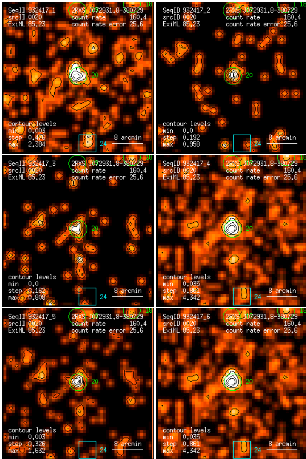
Figure 20: RASS 932417: detection 0020: band rate images, Gaussian filter: (1) PSPC channels 11 – 41, (2) 52 – 90, (3) 91 – 201, (4) 11 – 235, (5) 52 – 201, (6) 11 – 201. Broad band rates in counts/ks. Band rate contour levels in counts/ks/arcmin 2 .
