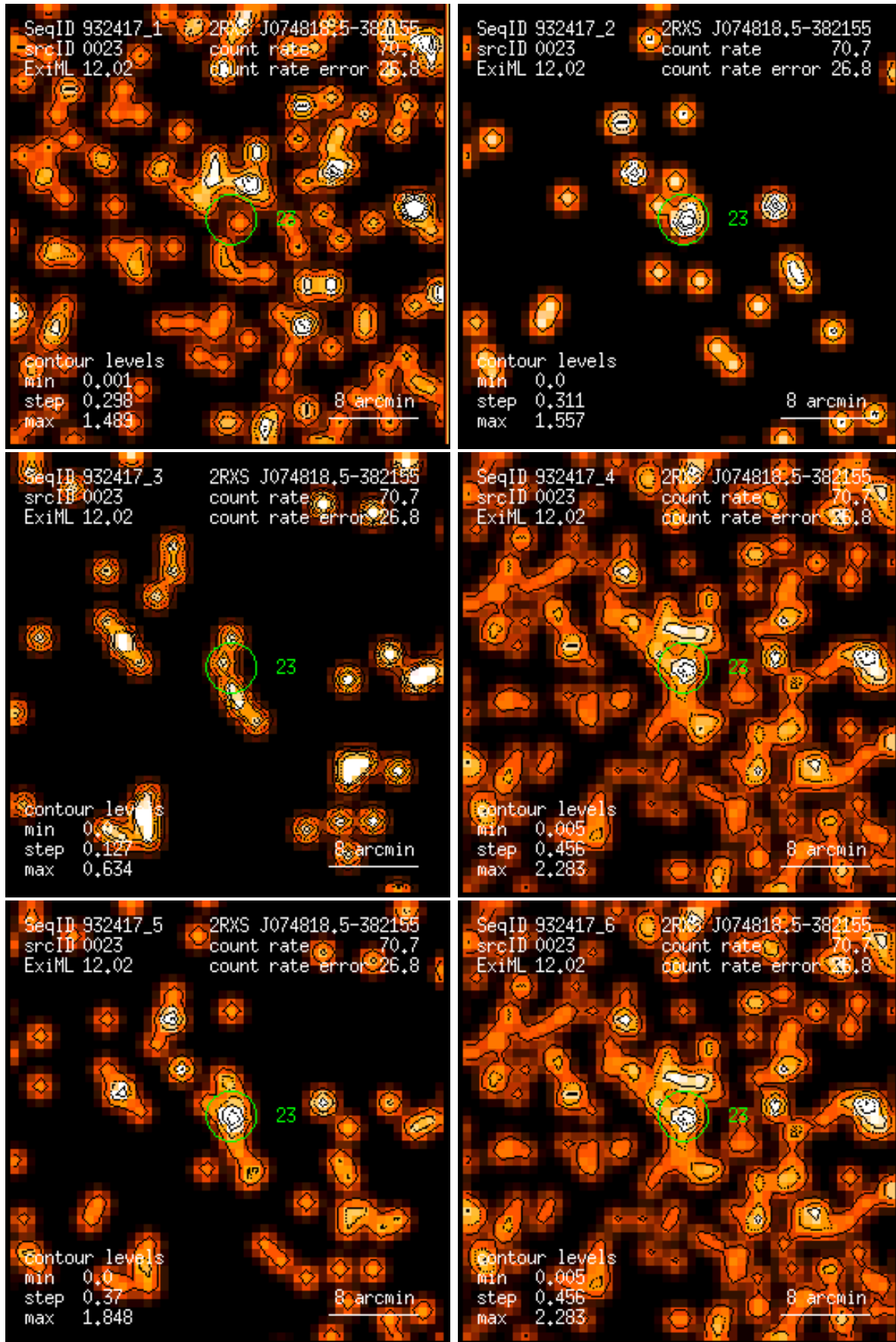
Figure 23: RASS 932417: detection 0023: band rate images, Gaussian filter: (1) PSPC channels 11 – 41, (2) 52 – 90, (3) 91 – 201, (4) 11 – 235, (5) 52 – 201, (6) 11 – 201. Broad band rates in counts/ks. Band rate contour levels in counts/ks/arcmin 2 .
