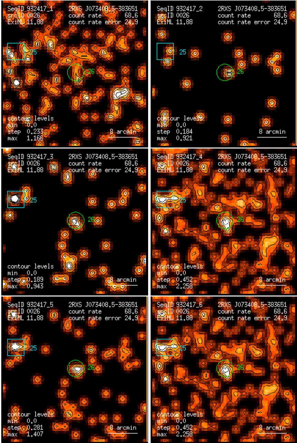
Figure 26: RASS 932417: detection 0026: band rate images, Gaussian filter: (1) PSPC channels 11 – 41, (2) 52 – 90, (3) 91 – 201, (4) 11 – 235, (5) 52 – 201, (6) 11 – 201. Broad band rates in counts/ks. Band rate contour levels in counts/ks/arcmin 2 .
