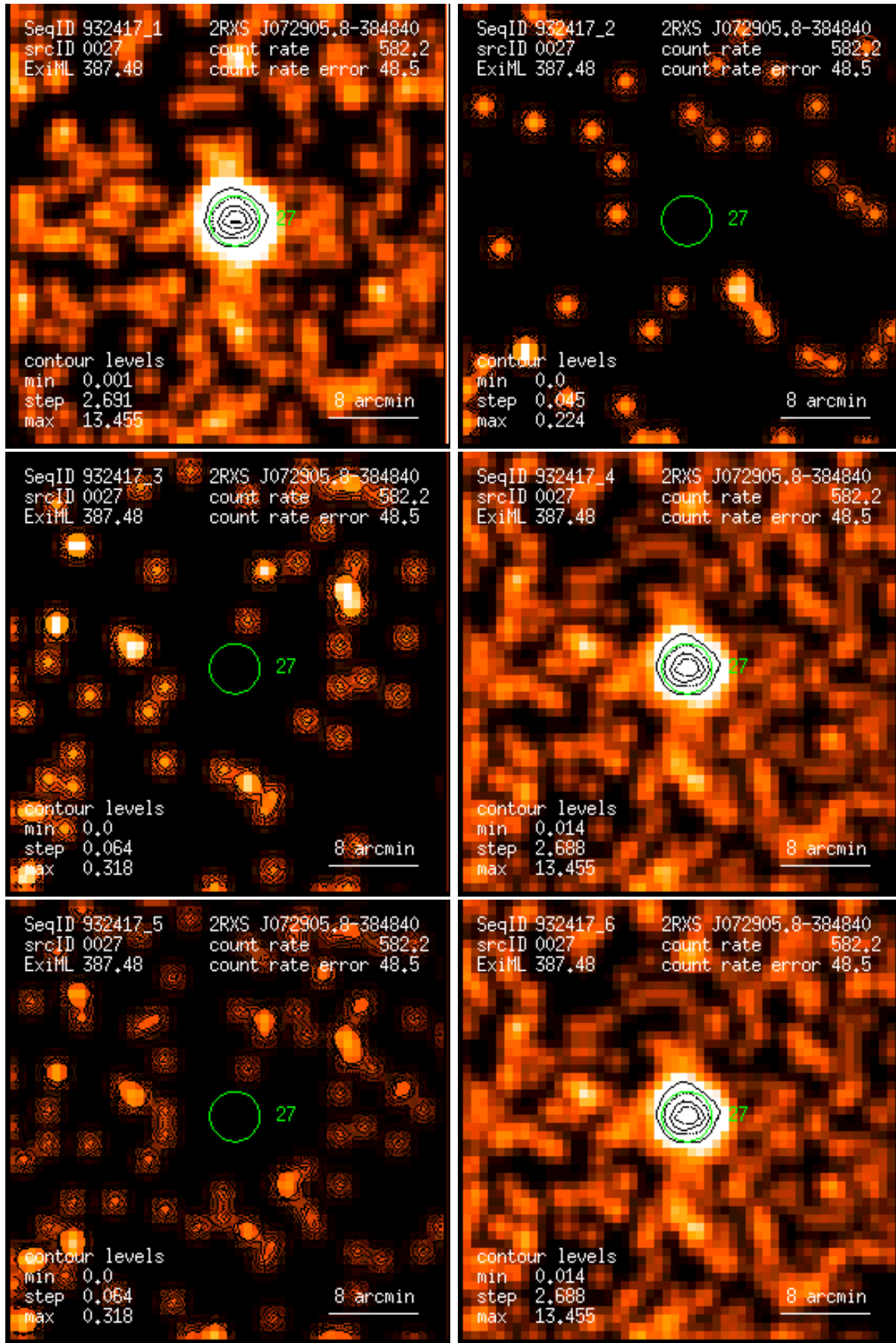
Figure 27: RASS 932417: detection 0027: band rate images, Gaussian filter: (1) PSPC channels 11 – 41, (2) 52 – 90, (3) 91 – 201, (4) 11 – 235, (5) 52 – 201, (6) 11 – 201. Broad band rates in counts/ks. Band rate contour levels in counts/ks/arcmin 2 .
