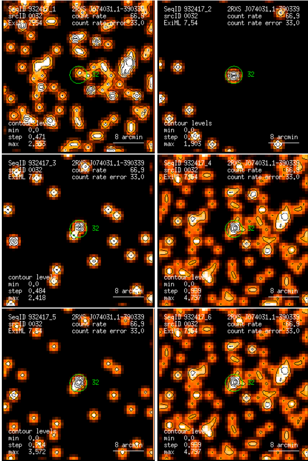
Figure 32: RASS 932417: detection 0032: band rate images, Gaussian filter: (1) PSPC channels 11 – 41, (2) 52 – 90, (3) 91 – 201, (4) 11 – 235, (5) 52 – 201, (6) 11 – 201. Broad band rates in counts/ks. Band rate contour levels in counts/ks/arcmin 2 .
