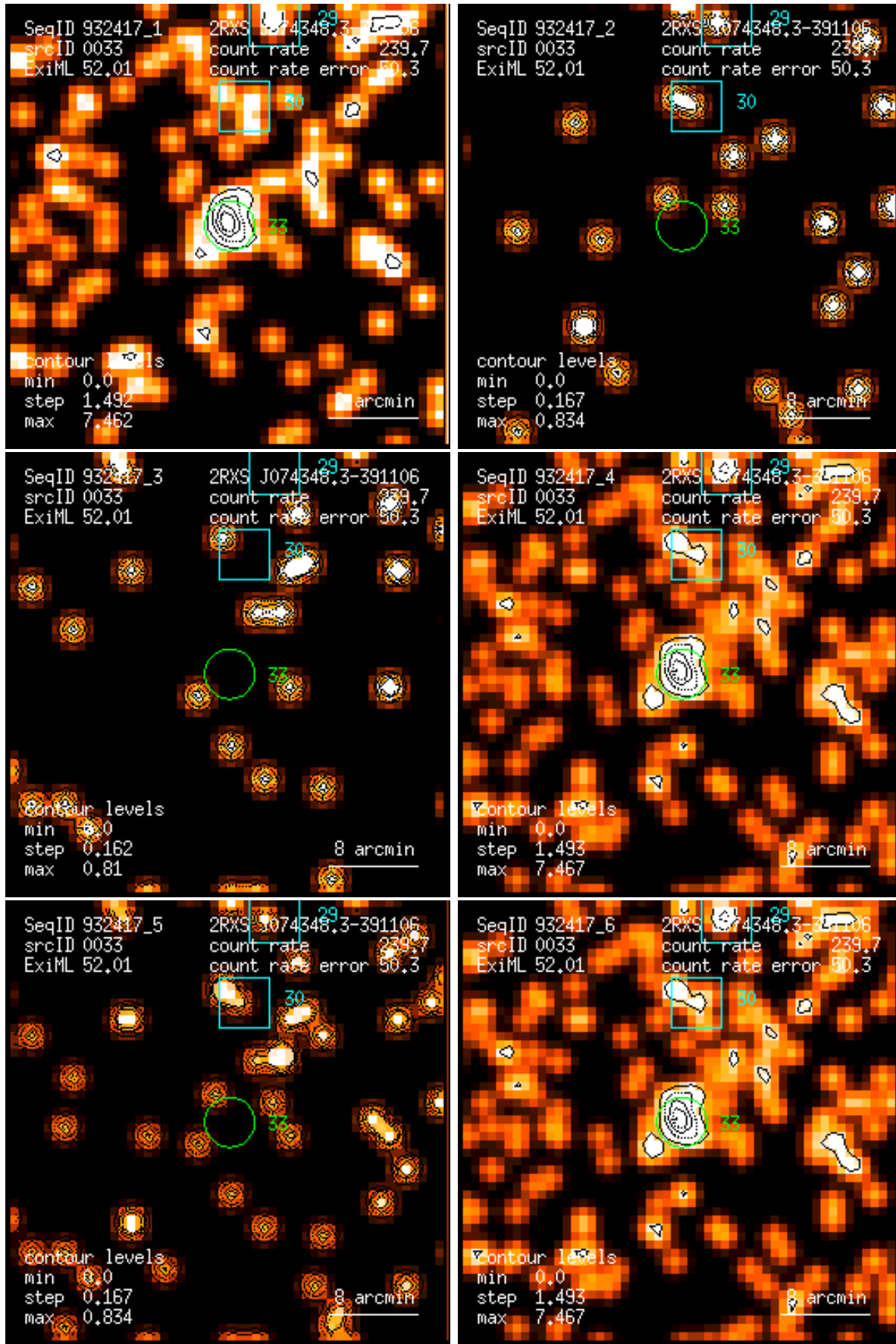
Figure 33: RASS 932417: detection 0033: band rate images, Gaussian filter: (1) PSPC channels 11 – 41, (2) 52 – 90, (3) 91 – 201, (4) 11 – 235, (5) 52 – 201, (6) 11 – 201. Broad band rates in counts/ks. Band rate contour levels in counts/ks/arcmin 2 .
