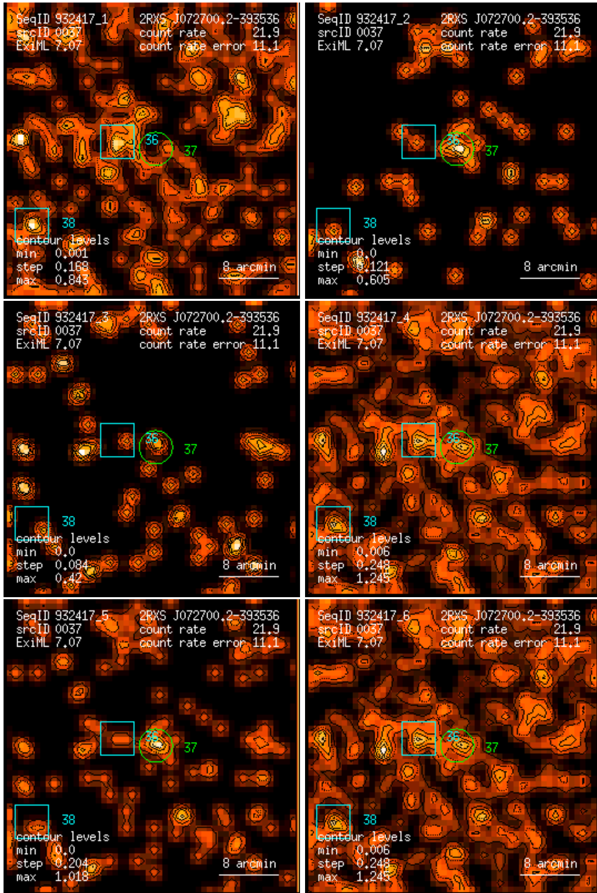
Figure 37: RASS 932417: detection 0037: band rate images, Gaussian filter: (1) PSPC channels 11 – 41, (2) 52 – 90, (3) 91 – 201, (4) 11 – 235, (5) 52 – 201, (6) 11 – 201. Broad band rates in counts/ks. Band rate contour levels in counts/ks/arcmin 2 .
