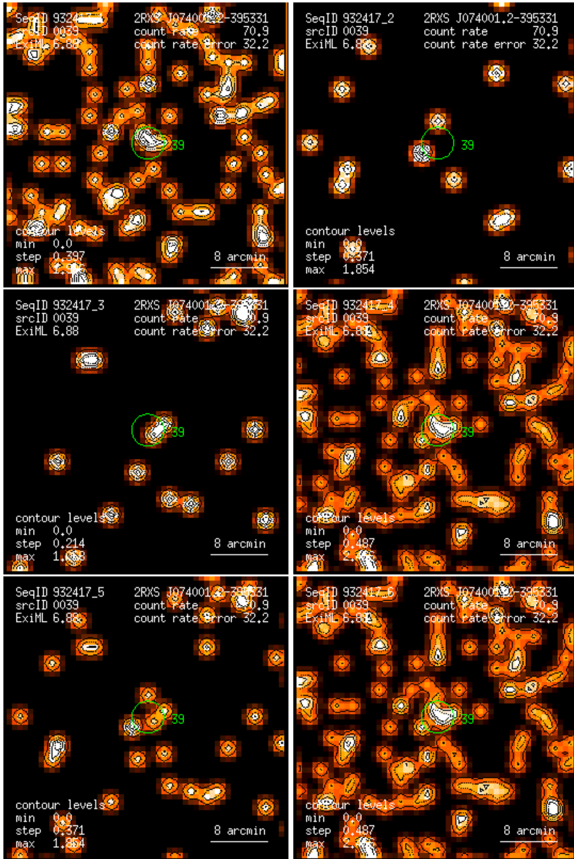
Figure 39: RASS 932417: detection 0039: band rate images, Gaussian filter: (1) PSPC channels 11 – 41, (2) 52 – 90, (3) 91 – 201, (4) 11 – 235, (5) 52 – 201, (6) 11 – 201. Broad band rates in counts/ks. Band rate contour levels in counts/ks/arcmin 2 .
