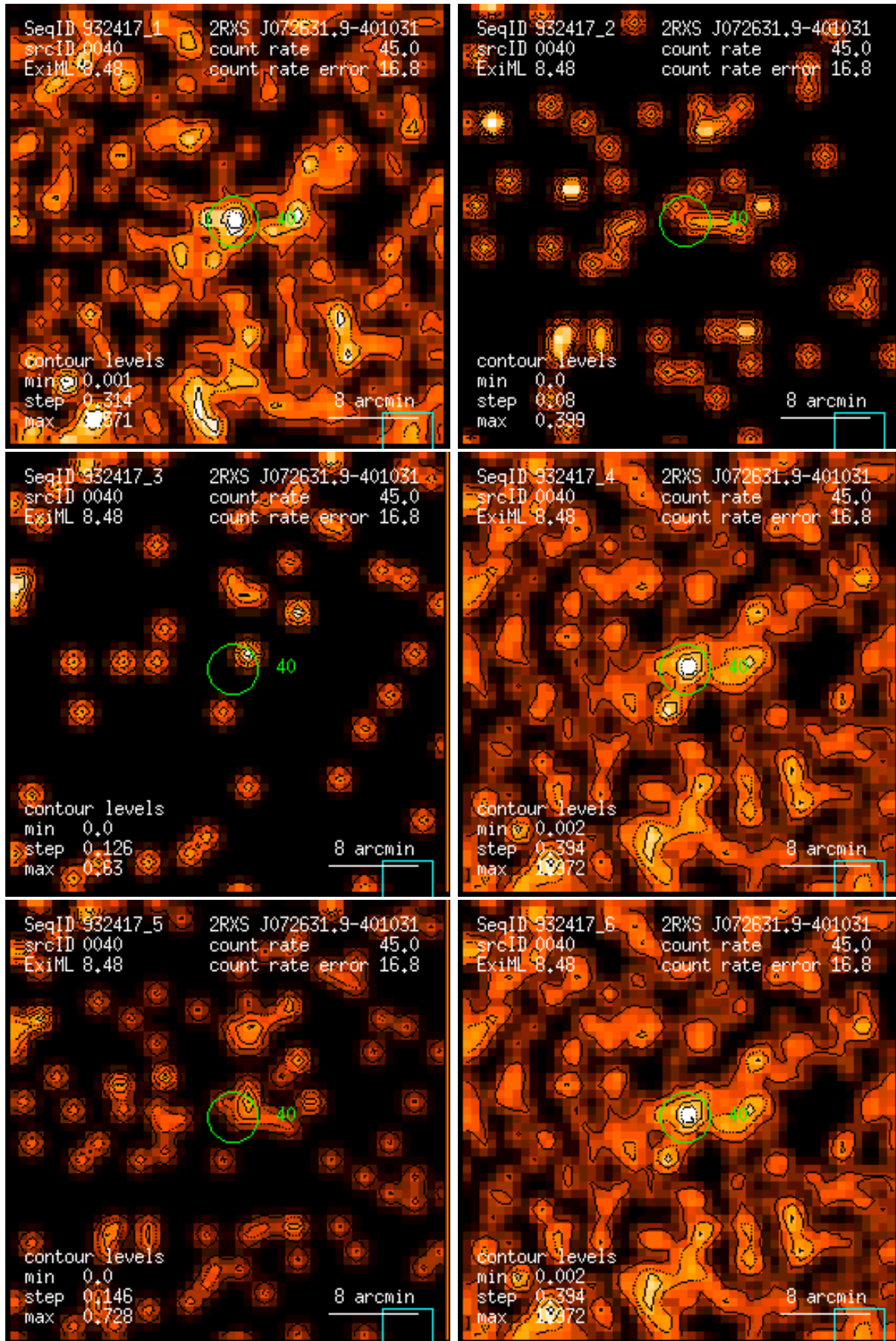
Figure 40: RASS 932417: detection 0040: band rate images, Gaussian filter: (1) PSPC channels 11 – 41, (2) 52 – 90, (3) 91 – 201, (4) 11 – 235, (5) 52 – 201, (6) 11 – 201. Broad band rates in counts/ks. Band rate contour levels in counts/ks/arcmin 2 .
