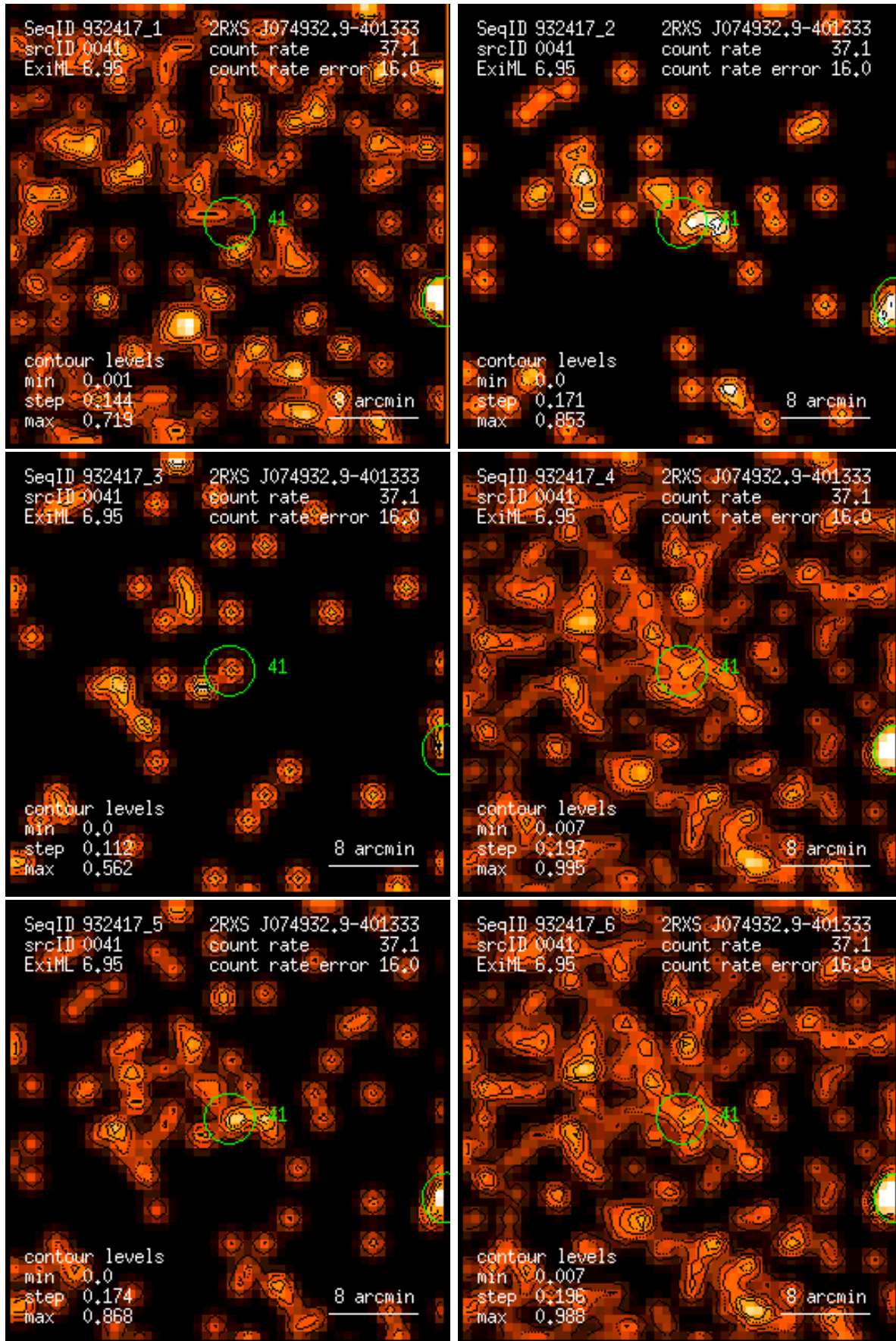
Figure 41: RASS 932417: detection 0041: band rate images, Gaussian filter: (1) PSPC channels 11 – 41, (2) 52 – 90, (3) 91 – 201, (4) 11 – 235, (5) 52 – 201, (6) 11 – 201. Broad band rates in counts/ks. Band rate contour levels in counts/ks/arcmin 2 .
