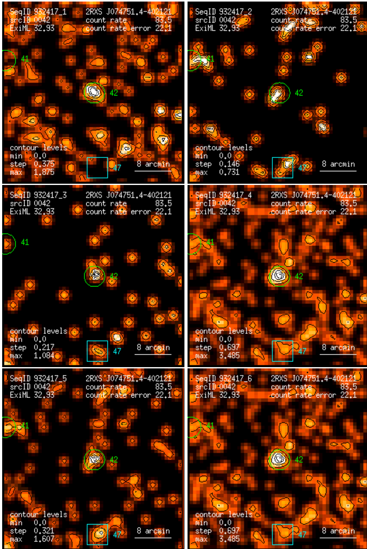
Figure 42: RASS 932417: detection 0042: band rate images, Gaussian filter: (1) PSPC channels 11 – 41, (2) 52 – 90, (3) 91 – 201, (4) 11 – 235, (5) 52 – 201, (6) 11 – 201. Broad band rates in counts/ks. Band rate contour levels in counts/ks/arcmin 2 .
