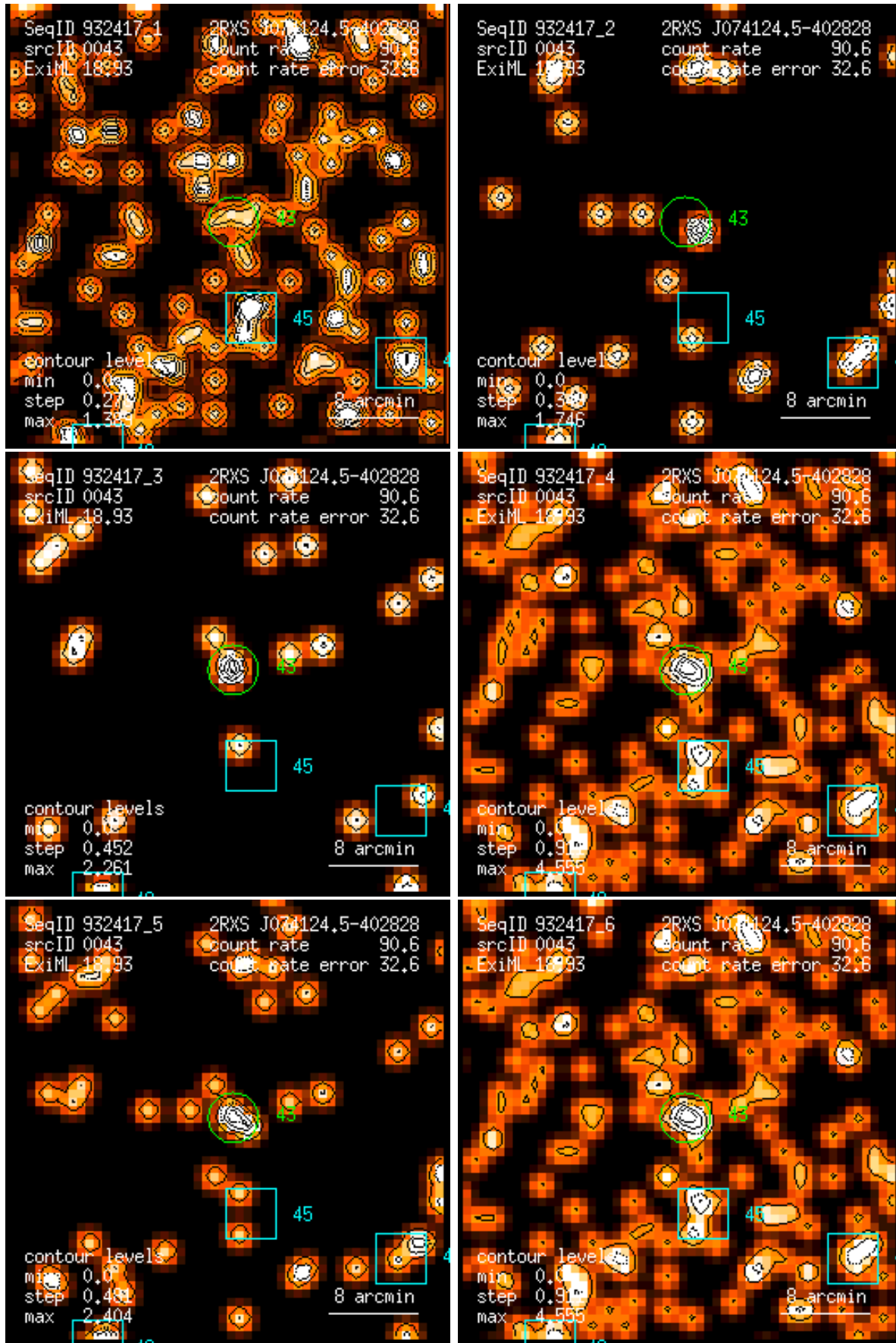
Figure 43: RASS 932417: detection 0043: band rate images, Gaussian filter: (1) PSPC channels 11 – 41, (2) 52 – 90, (3) 91 – 201, (4) 11 – 235, (5) 52 – 201, (6) 11 – 201. Broad band rates in counts/ks. Band rate contour levels in counts/ks/arcmin 2 .
