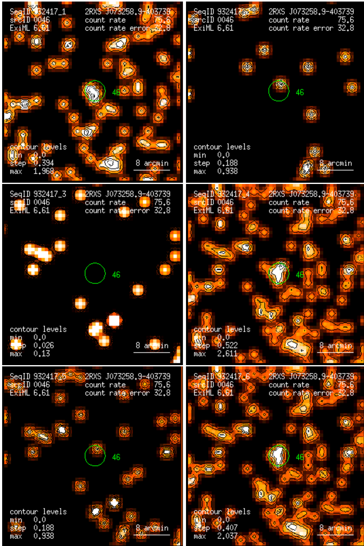
Figure 46: RASS 932417: detection 0046: band rate images, Gaussian filter: (1) PSPC channels 11 – 41, (2) 52 – 90, (3) 91 – 201, (4) 11 – 235, (5) 52 – 201, (6) 11 – 201. Broad band rates in counts/ks. Band rate contour levels in counts/ks/arcmin 2 .
