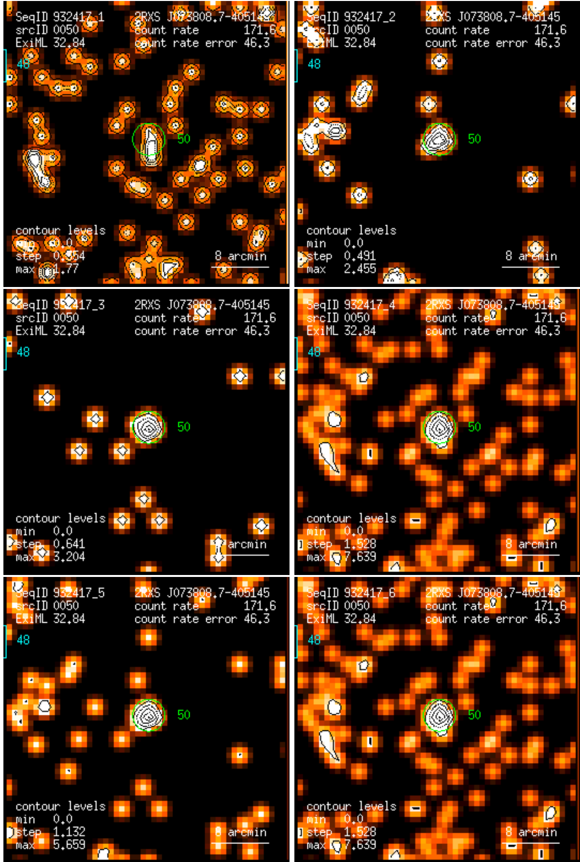
Figure 50: RASS 932417: detection 0050: band rate images, Gaussian filter: (1) PSPC channels 11 – 41, (2) 52 – 90, (3) 91 – 201, (4) 11 – 235, (5) 52 – 201, (6) 11 – 201. Broad band rates in counts/ks. Band rate contour levels in counts/ks/arcmin 2 .
