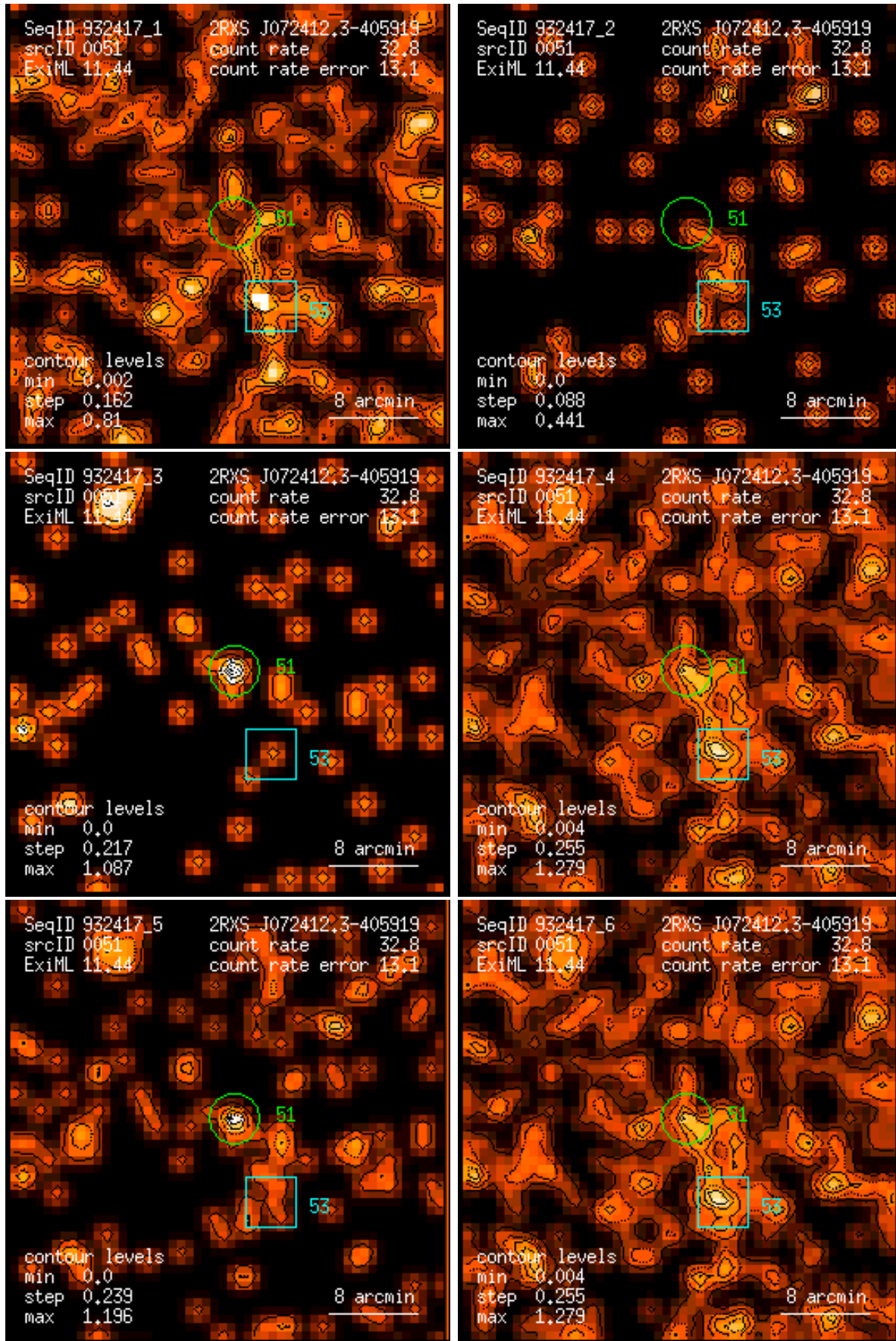
Figure 51: RASS 932417: detection 0051: band rate images, Gaussian filter: (1) PSPC channels 11 – 41, (2) 52 – 90, (3) 91 – 201, (4) 11 – 235, (5) 52 – 201, (6) 11 – 201. Broad band rates in counts/ks. Band rate contour levels in counts/ks/arcmin 2 .
