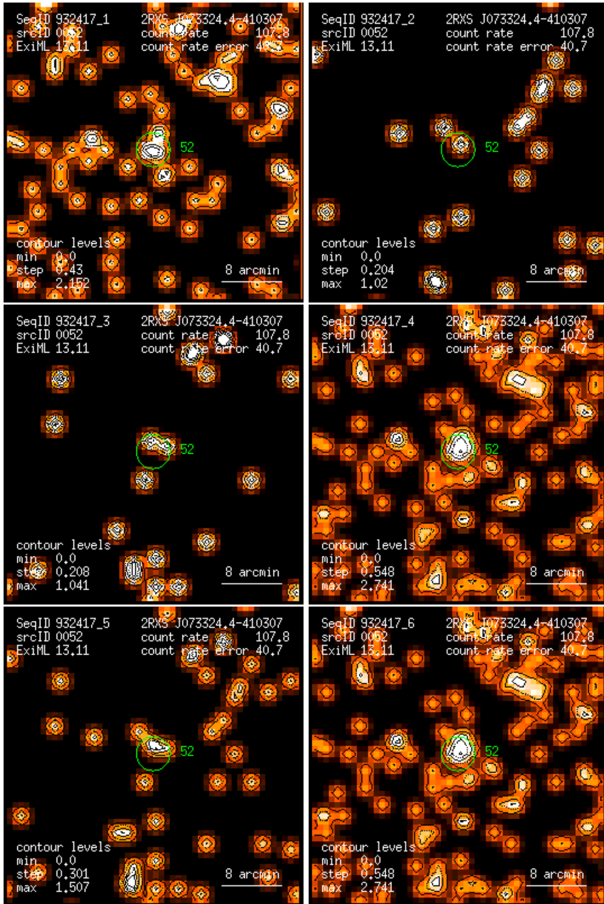
Figure 52: RASS 932417: detection 0052: band rate images, Gaussian filter: (1) PSPC channels 11 – 41, (2) 52 – 90, (3) 91 – 201, (4) 11 – 235, (5) 52 – 201, (6) 11 – 201. Broad band rates in counts/ks. Band rate contour levels in counts/ks/arcmin 2 .
