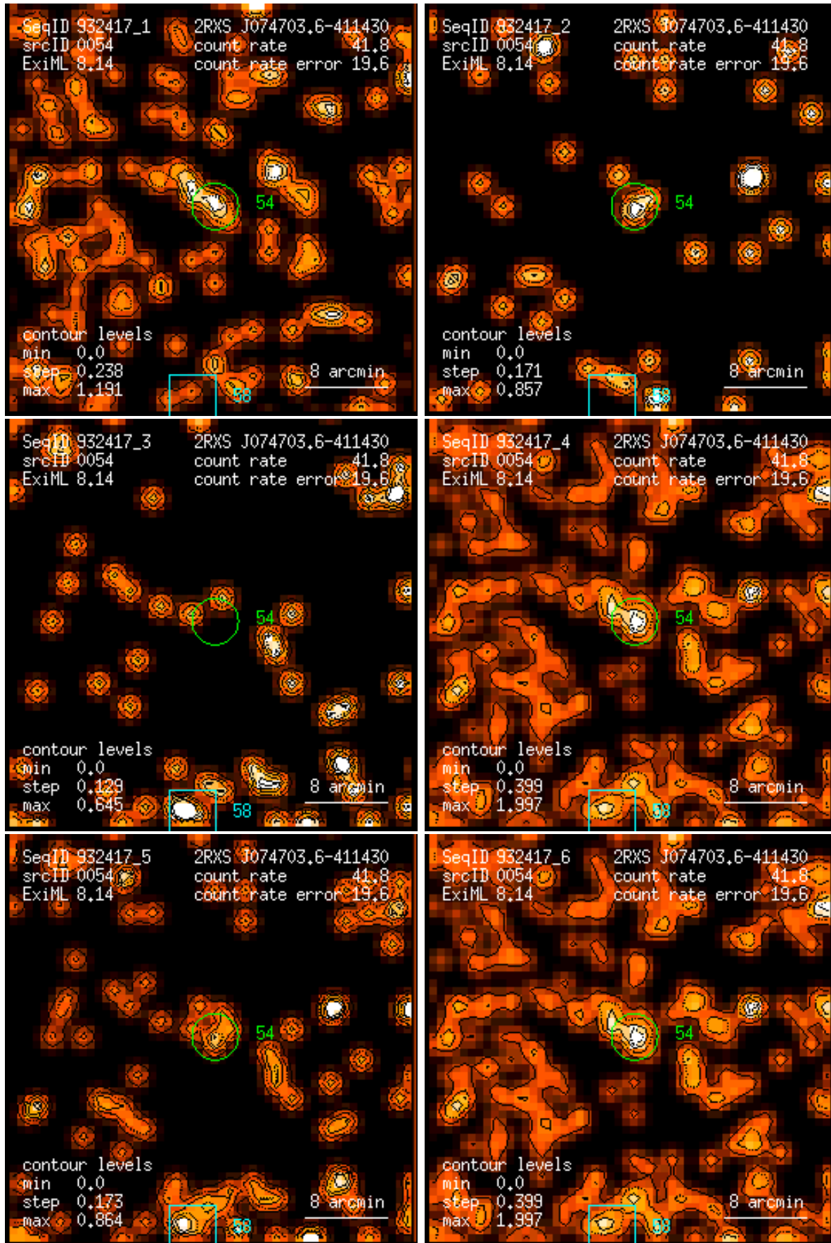
Figure 54: RASS 932417: detection 0054: band rate images, Gaussian filter: (1) PSPC channels 11 – 41, (2) 52 – 90, (3) 91 – 201, (4) 11 – 235, (5) 52 – 201, (6) 11 – 201. Broad band rates in counts/ks. Band rate contour levels in counts/ks/arcmin 2 .
