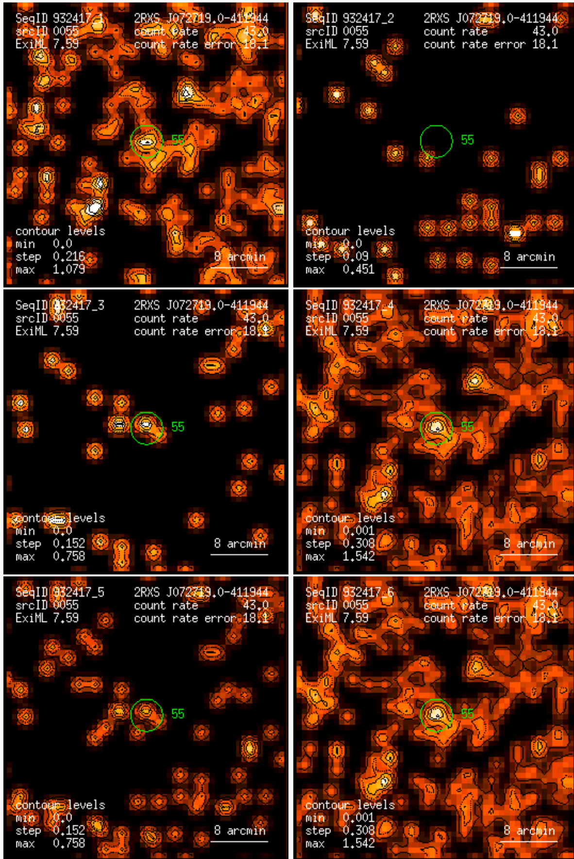
Figure 55: RASS 932417: detection 0055: band rate images, Gaussian filter: (1) PSPC channels 11 – 41, (2) 52 – 90, (3) 91 – 201, (4) 11 – 235, (5) 52 – 201, (6) 11 – 201. Broad band rates in counts/ks. Band rate contour levels in counts/ks/arcmin 2 .
